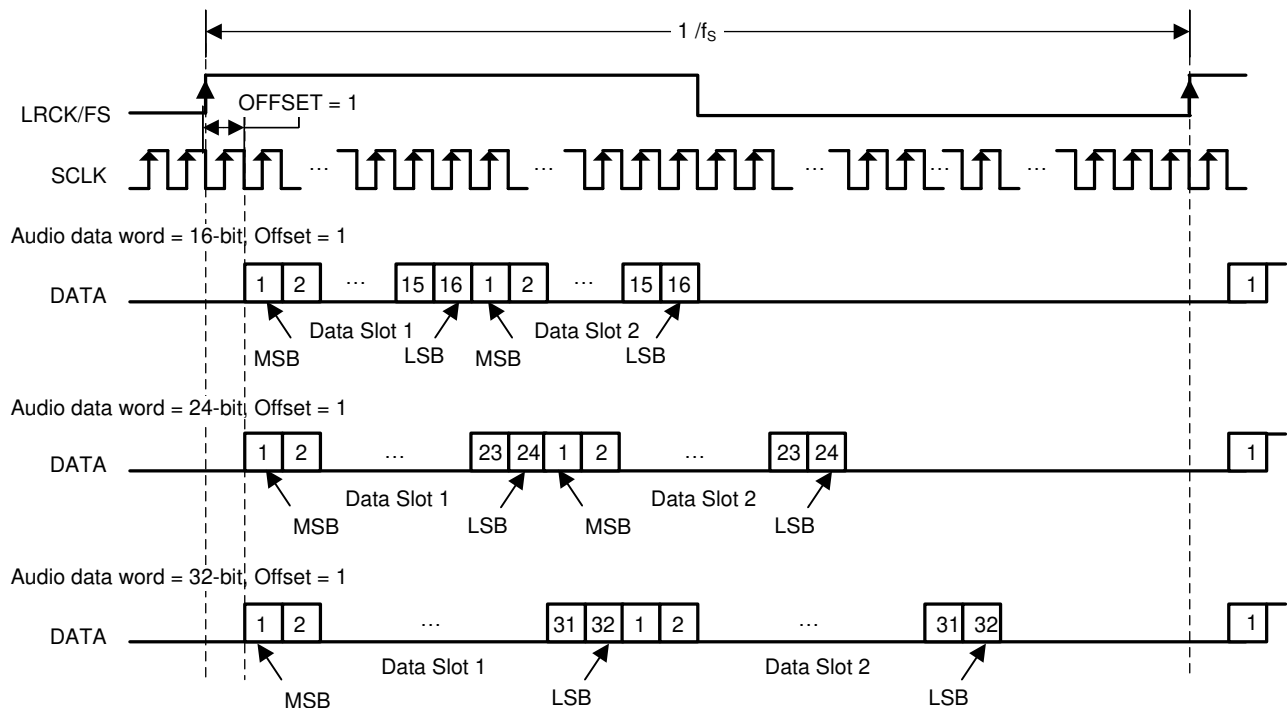
7-5. TDM 1 Audio Data Format
