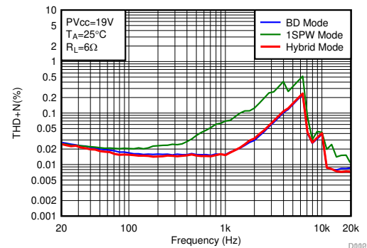
6-10. THD+N vs Frequency-BTL
