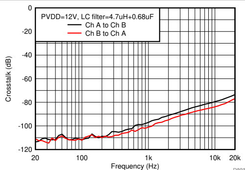
6-27. Crosstalk
