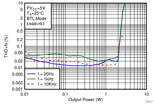
6-42. THD+N vs Output Power
