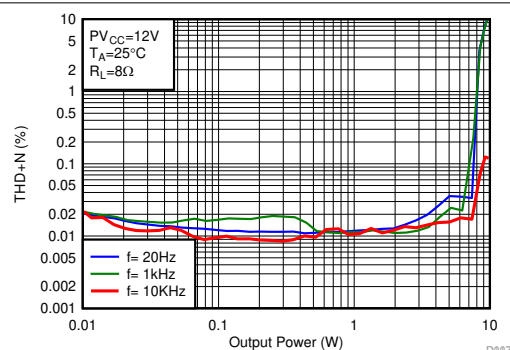
6-20. THD+N vs Output Power-BTL
