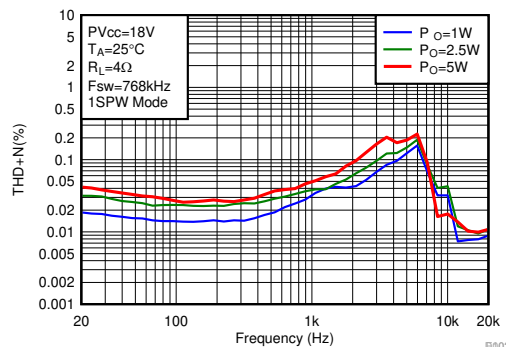
6-2. THD+N vs Frequency-BTL
