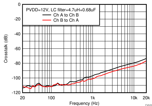
6-26. Crosstalk
