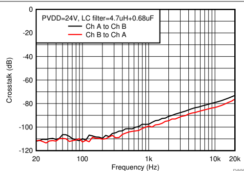
6-26. Crosstalk
