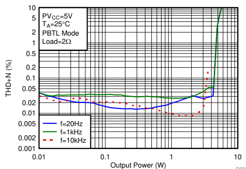
FIG 6-80. THD+N vs Output Power
