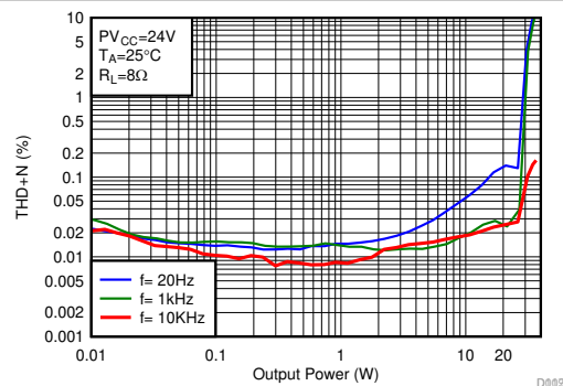
6-22. THD+N vs Output Power-BTL
