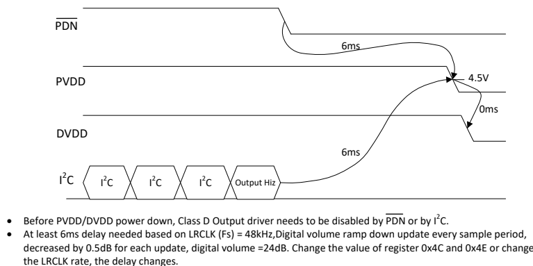
7-15. Power-Down Sequence
