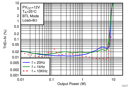
6-44. THD+N vs Output Power
