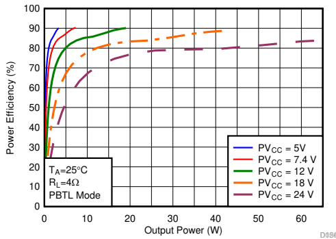
図 8-10. Efficiency vs Output Power (Inductor as Output Filter, Hybrid modulation, PBTL mode)
