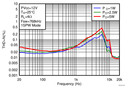
6-1. THD+N vs Frequency-BTL
