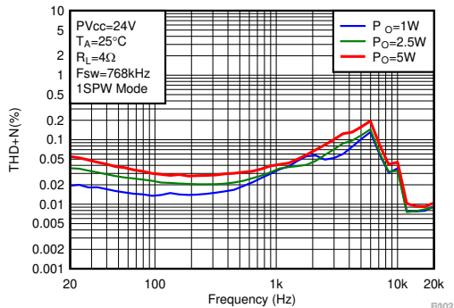
6-3. THD+N vs Frequency-BTL
