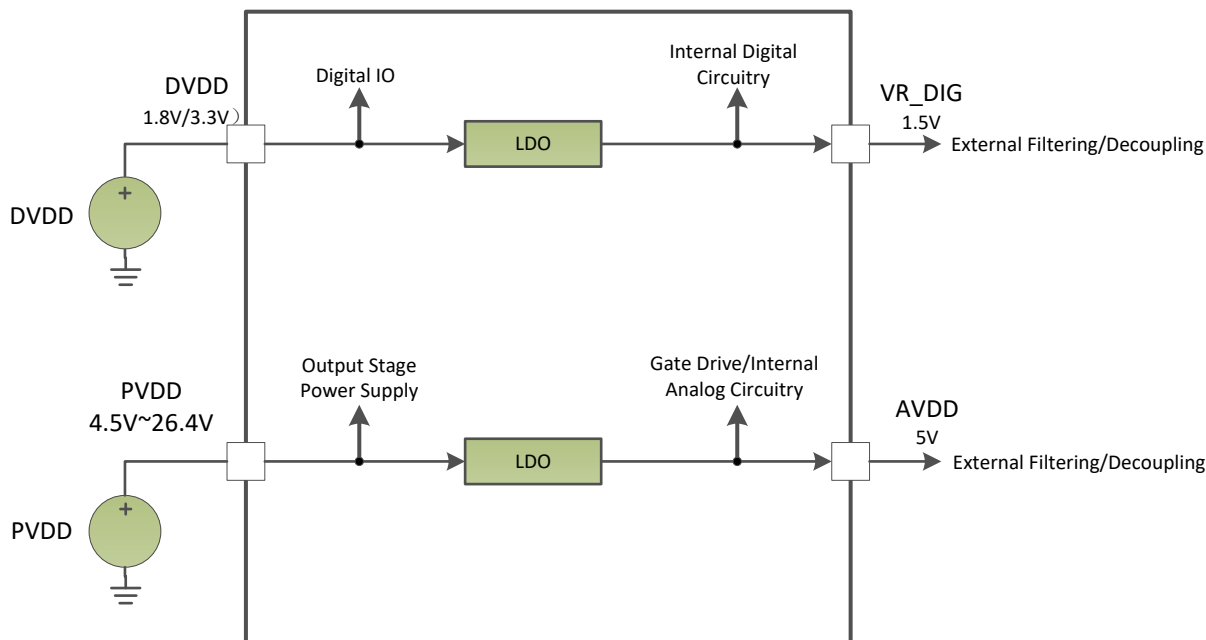
図 9-1. Power Supply Function Block Diagram
