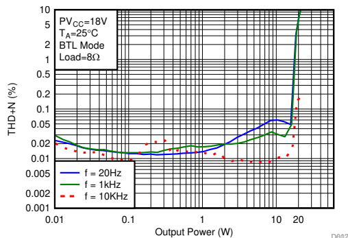
6-47. THD+N vs Output Power
