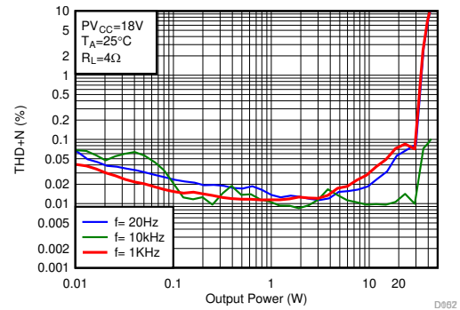
図 8-11. THD+N vs Output Power (Inductor as Output Filter, Hybrid Modulation, PBTL mode)
