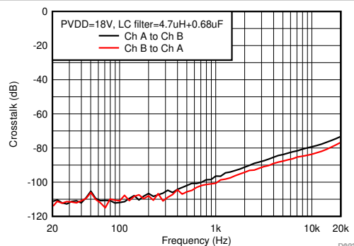
6-28. Crosstalk
