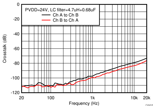
6-31. Crosstalk
