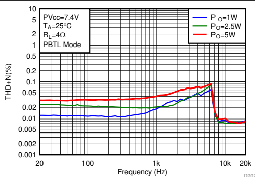
FIG 6-78. THD+N vs Frequency
