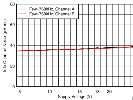
図 25. Idle Channel Noise vs Supply Voltage
