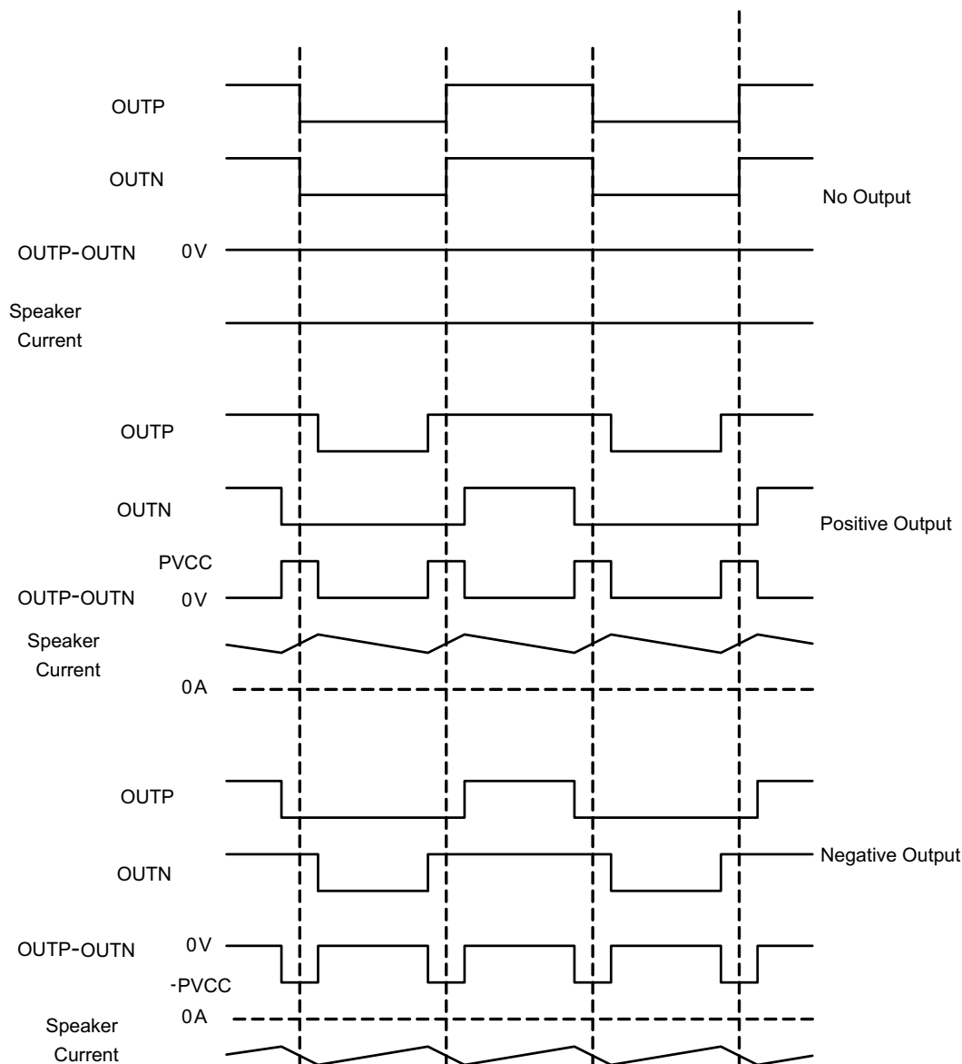
74. BD Mode Modulation
