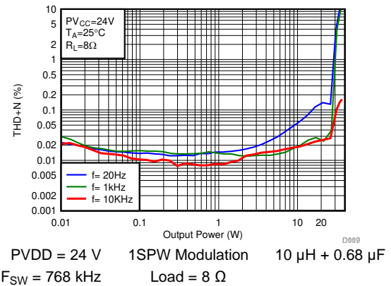
FIG 18. THD+N vs Output Power-BTL
