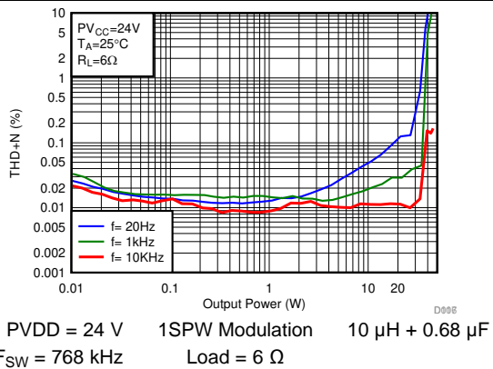
FIG 15. THD+N vs Output Power-BTL
