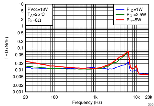
Figure 129. THD+N vs Frequency (1 SPW Mode, PVDD = 18 V, Load = 8 \Omega , BTL Mode)
