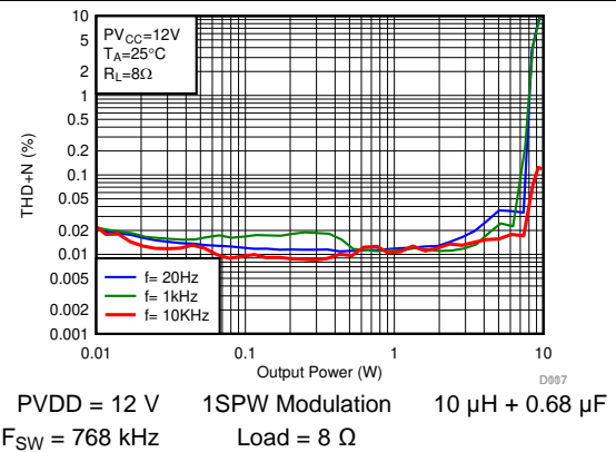
FIG 16. THD+N vs Output Power-BTL
