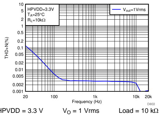
图 62. THD+N vs Frequency
