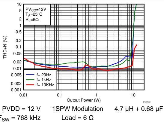
FIG 13. THD+N vs Output Power-BTL
