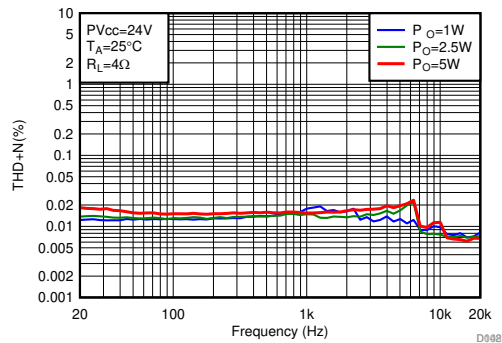
✕ 135. THD+N vs Frequency
