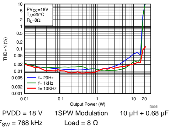
FIG 17. THD+N vs Output Power-BTL
