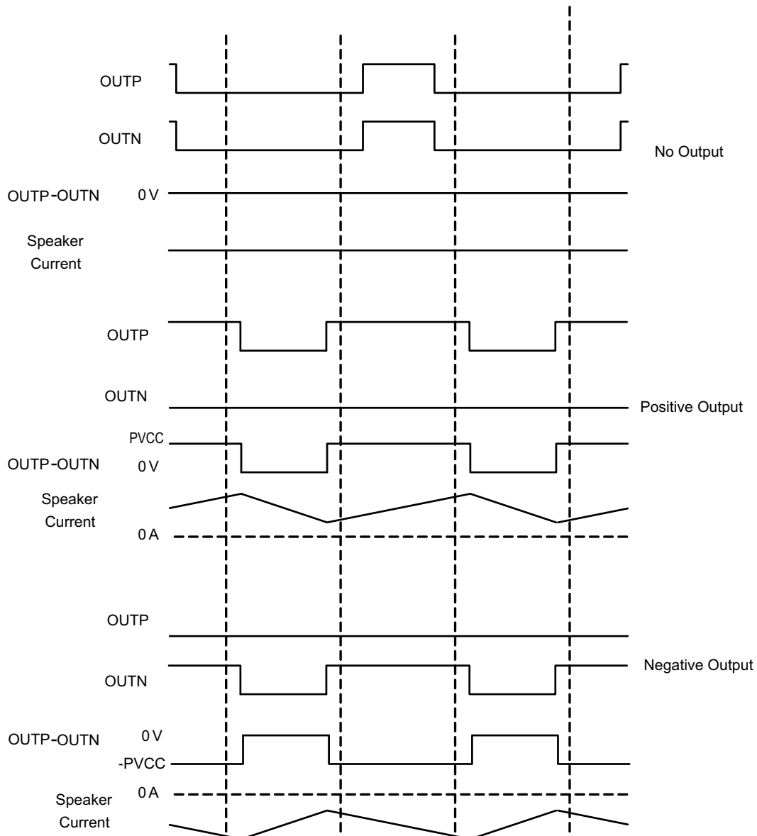
図 75. 1SPW Mode Modulation
