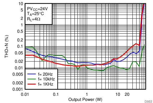
✕ 136. THD+N vs Output Power
