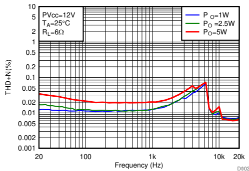
Figure 128. THD+N vs Frequency (1 SPW Mode, PVDD = 12 V, Load = 6 \Omega , BTL Mode)
