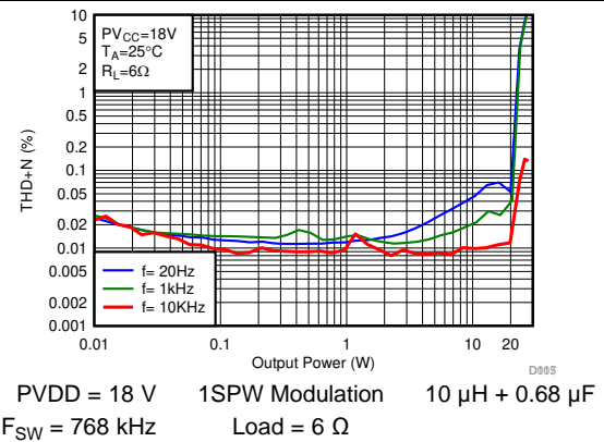
FIG 14. THD+N vs Output Power-BTL
