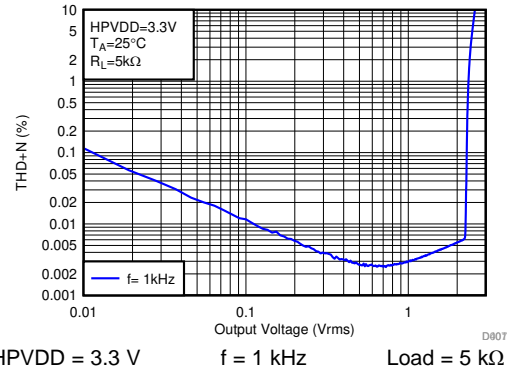
图 60. THD+N vs Output Voltage
