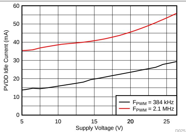
Figure 20. PVDD Current vs Voltage
