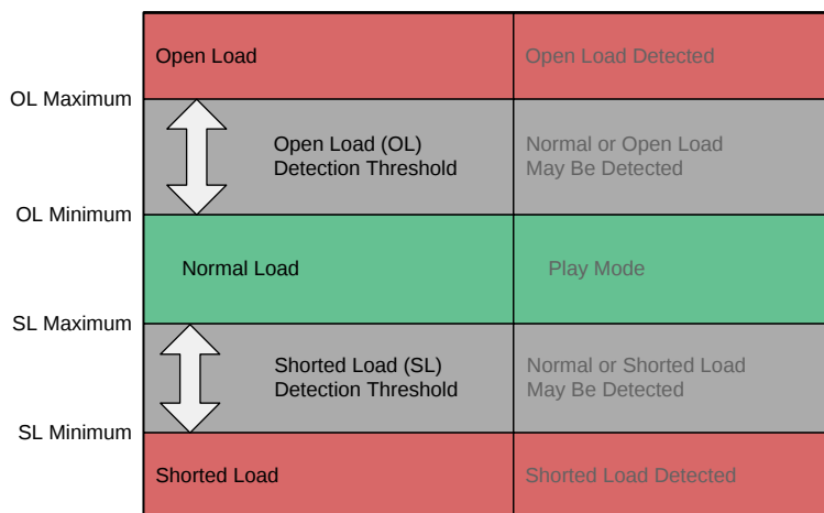
FIG 40. DC Load Diagnostic Reporting Thresholds
