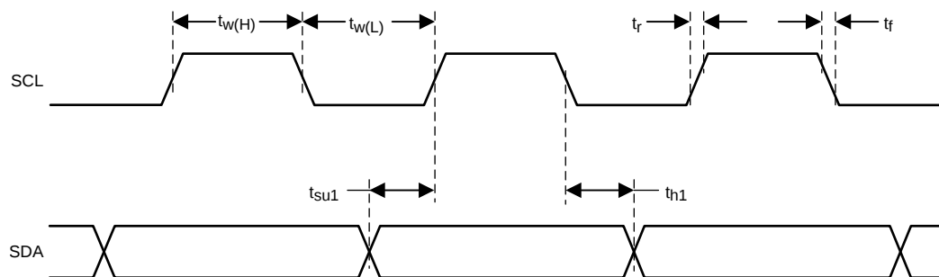
FIG 42. SCL and SDA Timing
