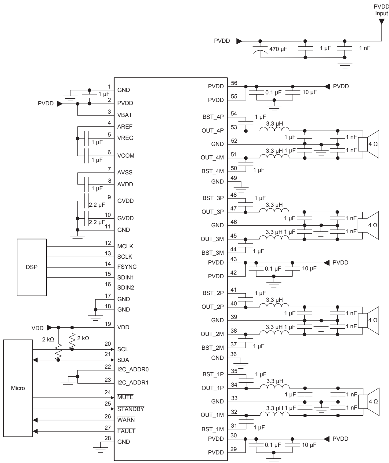
FIG 79. Typical 4-Channel BTL Application Schematic
