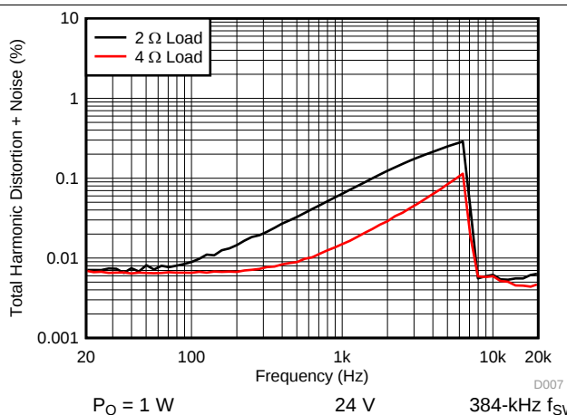
Figure 6. THD+N vs Frequency
