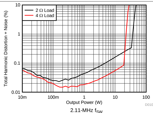
Figure 9. THD+N vs Power
