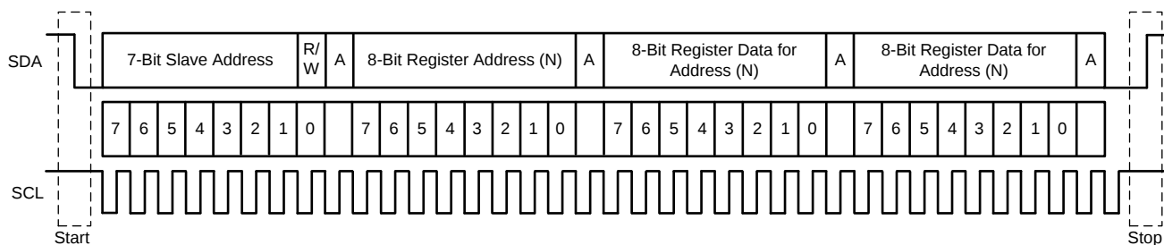
FIG 41. Typical I 2 C Sequence
