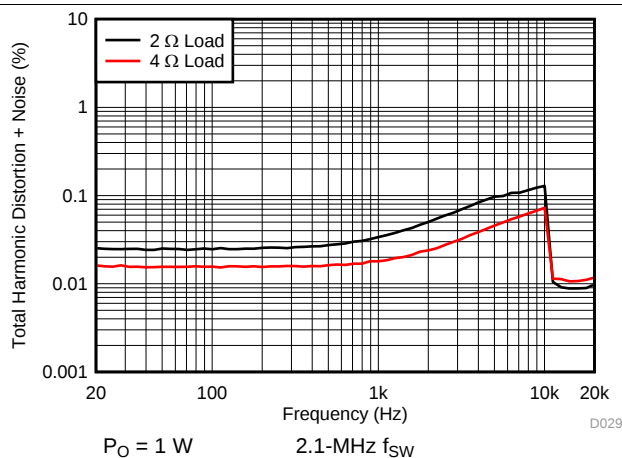
Figure 24. PBTL THD+N vs Frequency
