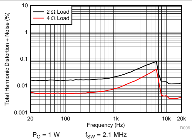
Figure 4. THD+N vs Frequency
