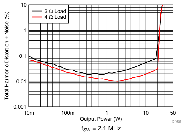
Figure 6. THD+N vs Power
