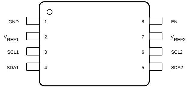
☒ 5-2. DCU Package, 8-Pin VSSOP, Top View
