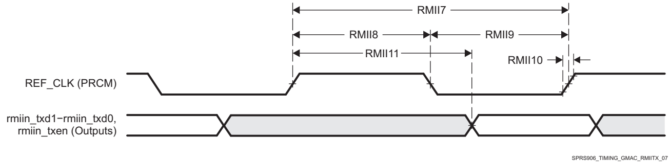
Figure 7-51. GMAC Transmit Interface Timing RMIIn Operation
