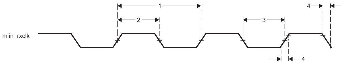
Figure 7-45. Clock Timing (GMAC Receive) - MII operation
