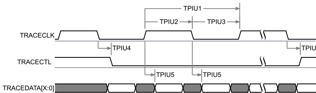
Figure 7-87. TPIU-PLL DDR Transmit Mode (1)
