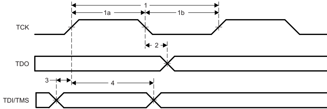
Figure 7-85. JTAG Timing
