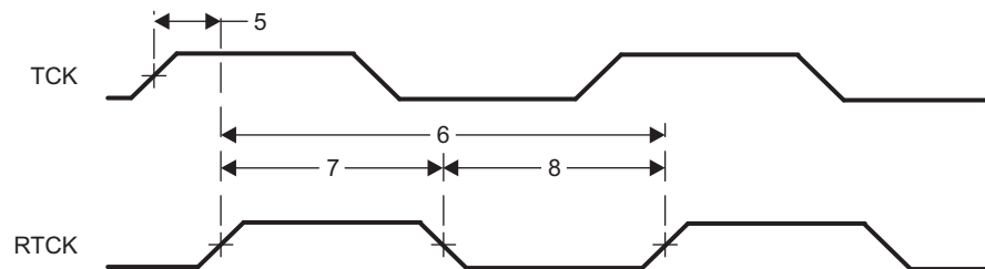
Figure 7-86. JTAG With RTCK Timing
