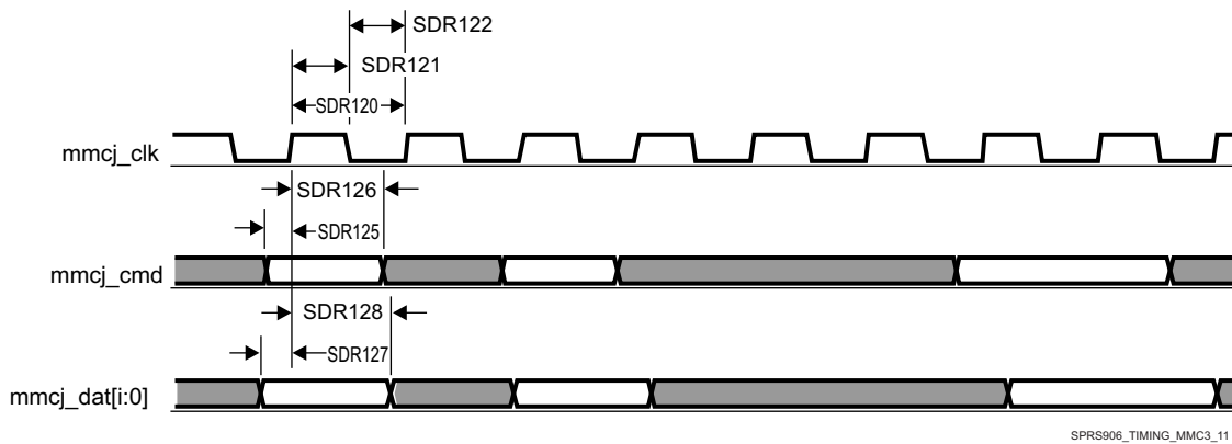
Figure 7-79. MMC/SD/SDIOj in - SDR12 - Receiver Mode
