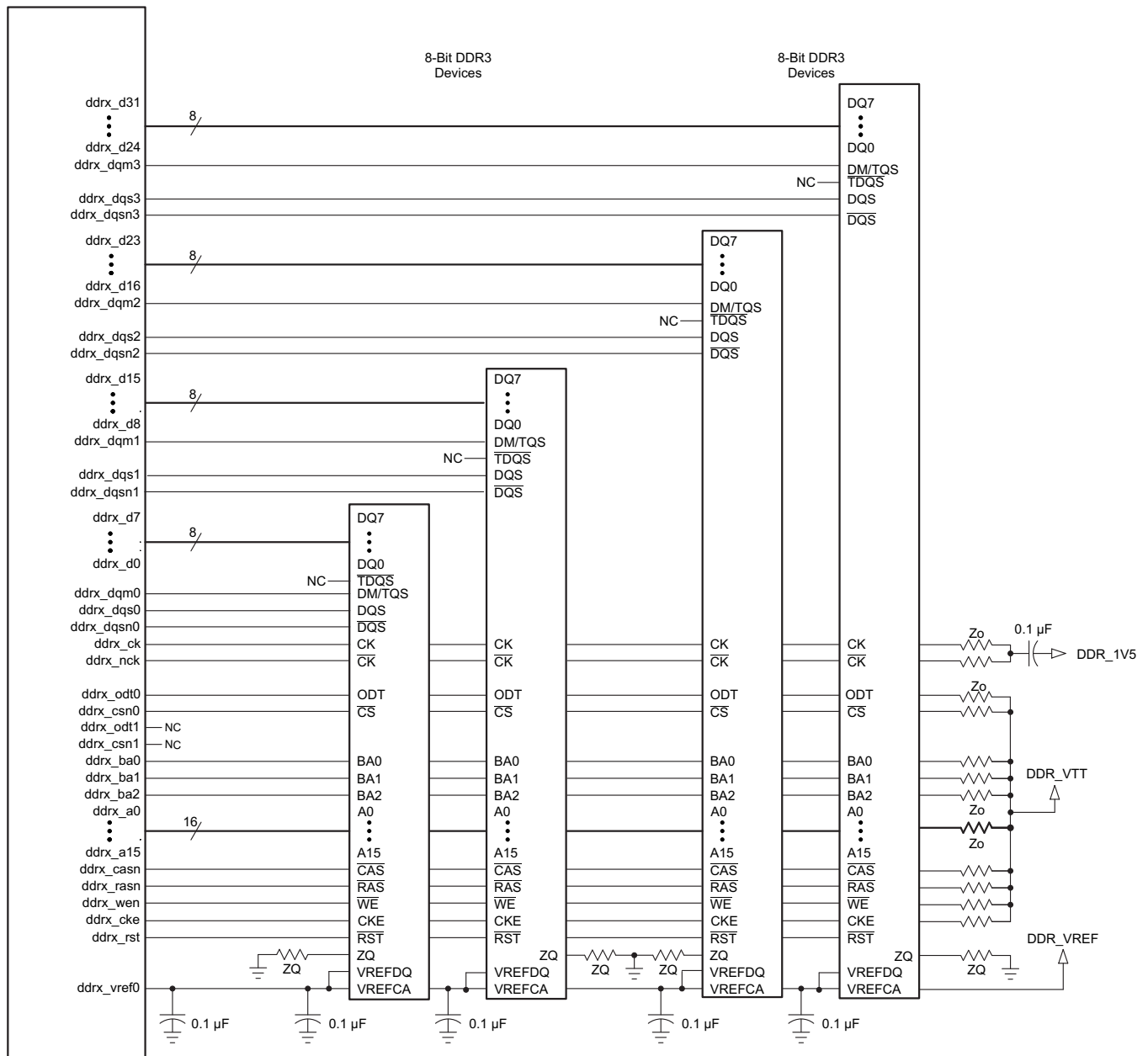
32-bit DDR3 EMIF
