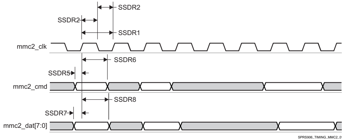
Figure 7-68. MMC/SD/SDIO in - Standard JC64 - Receiver Mode
