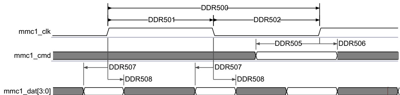
Figure 7-66. SDMMC - High Speed SD - DDR - Data/Command Receive
