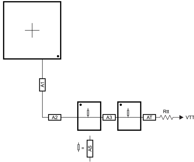
Figure 8-54. ADDR_CTRL Routing for Two Single-Side DDR3 Devices
