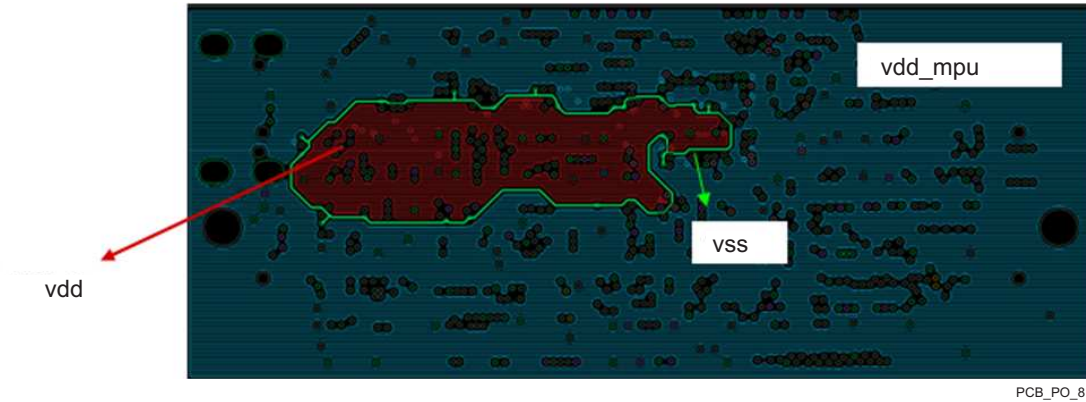
Figure 8-2. Coplanar Shielding of Power Net Using Ground Guard-band
