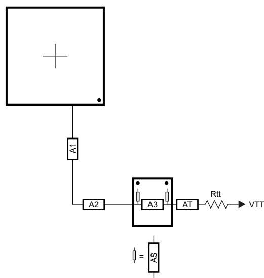
Figure 8-56. ADDR_CTRL Routing for Two Mirrored DDR3 Devices
