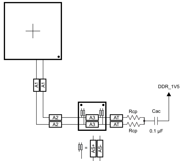
Figure 8-55. CK Routing for Two Mirrored DDR3 Devices
