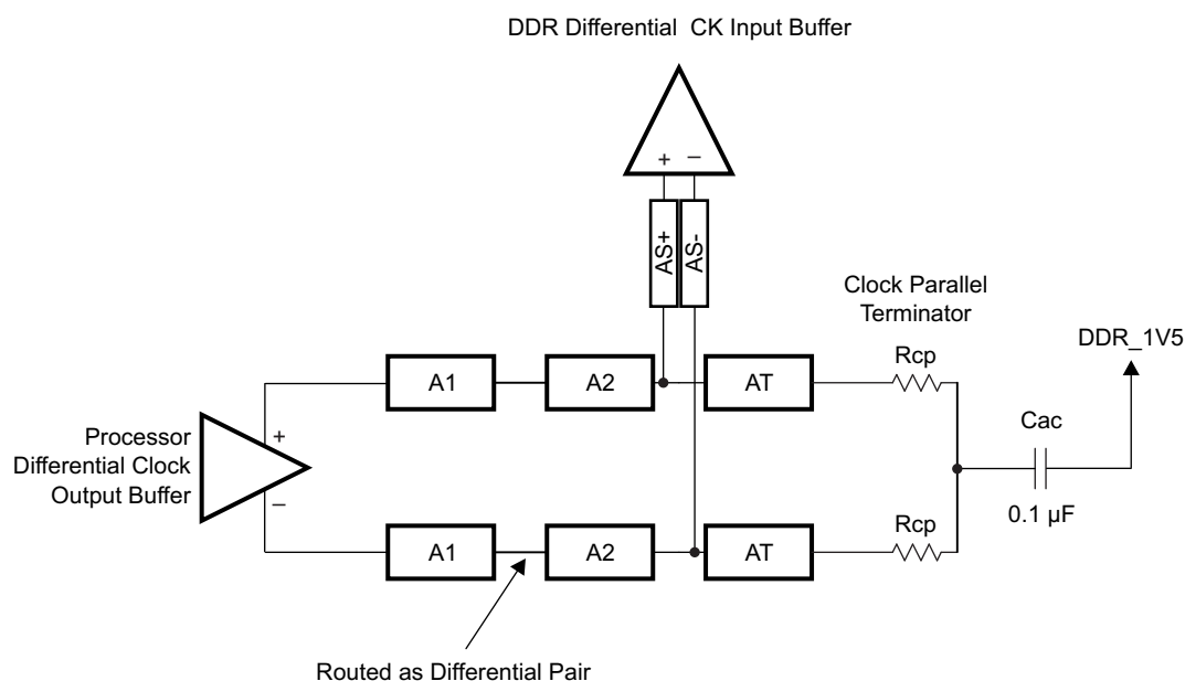
Figure 8-57. CK Topology for One DDR3 Device
