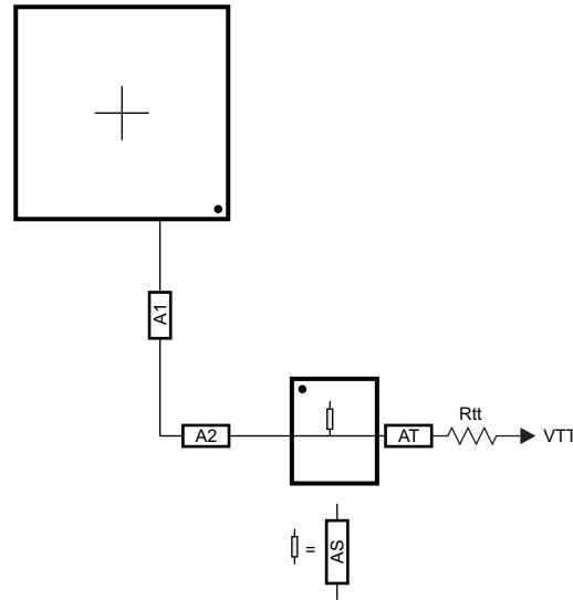
Figure 8-60. ADDR_CTRL Routing for One DDR3 Device
