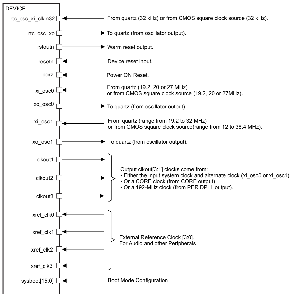
Figure 6-1. Clock Interface
