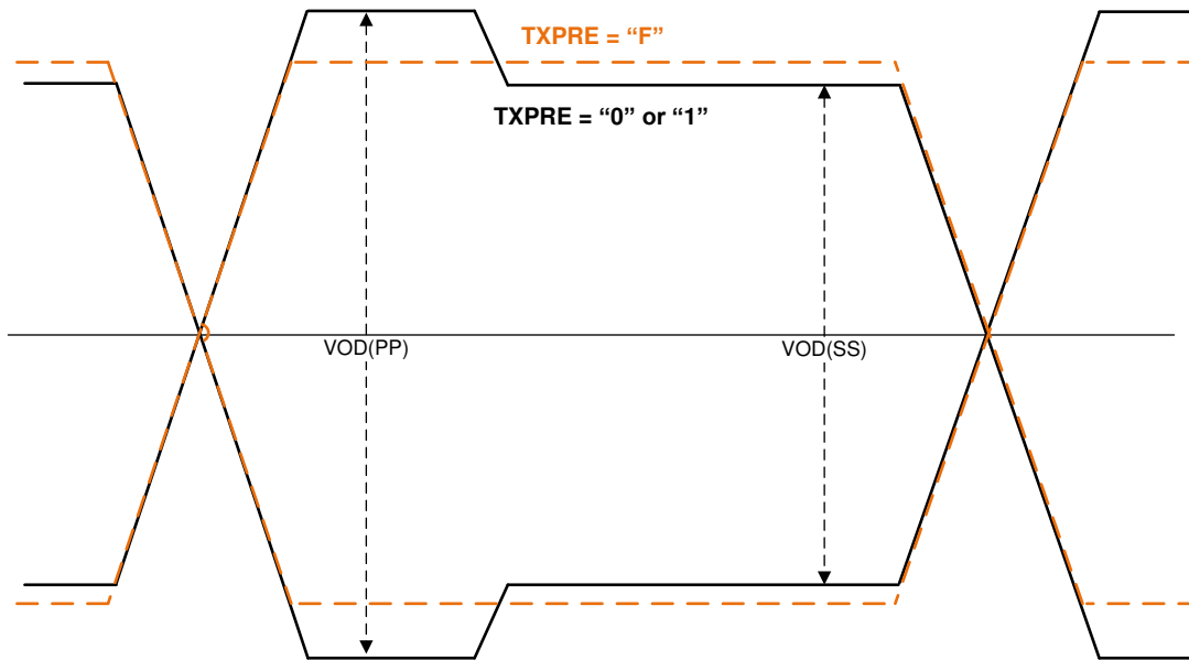
図 7-5. Output Differential Waveform with De-Emphasis
