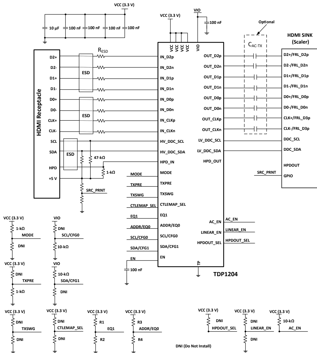
図 9-10. TDP1204 in Sink Application Schematics
