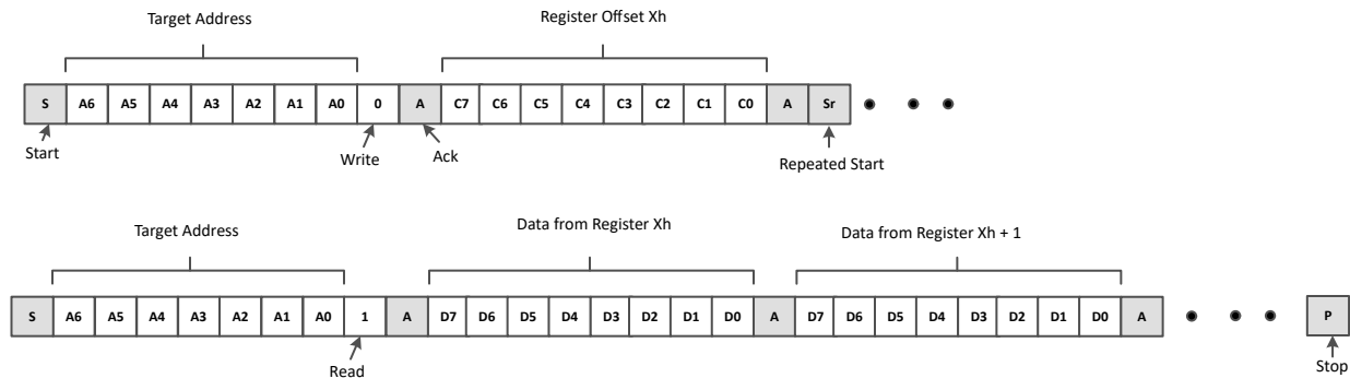
図 8-13. I2C Read with Repeated Start
