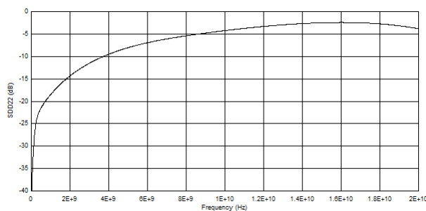
図 6-5. Output Differential Return Loss (SDD22)
