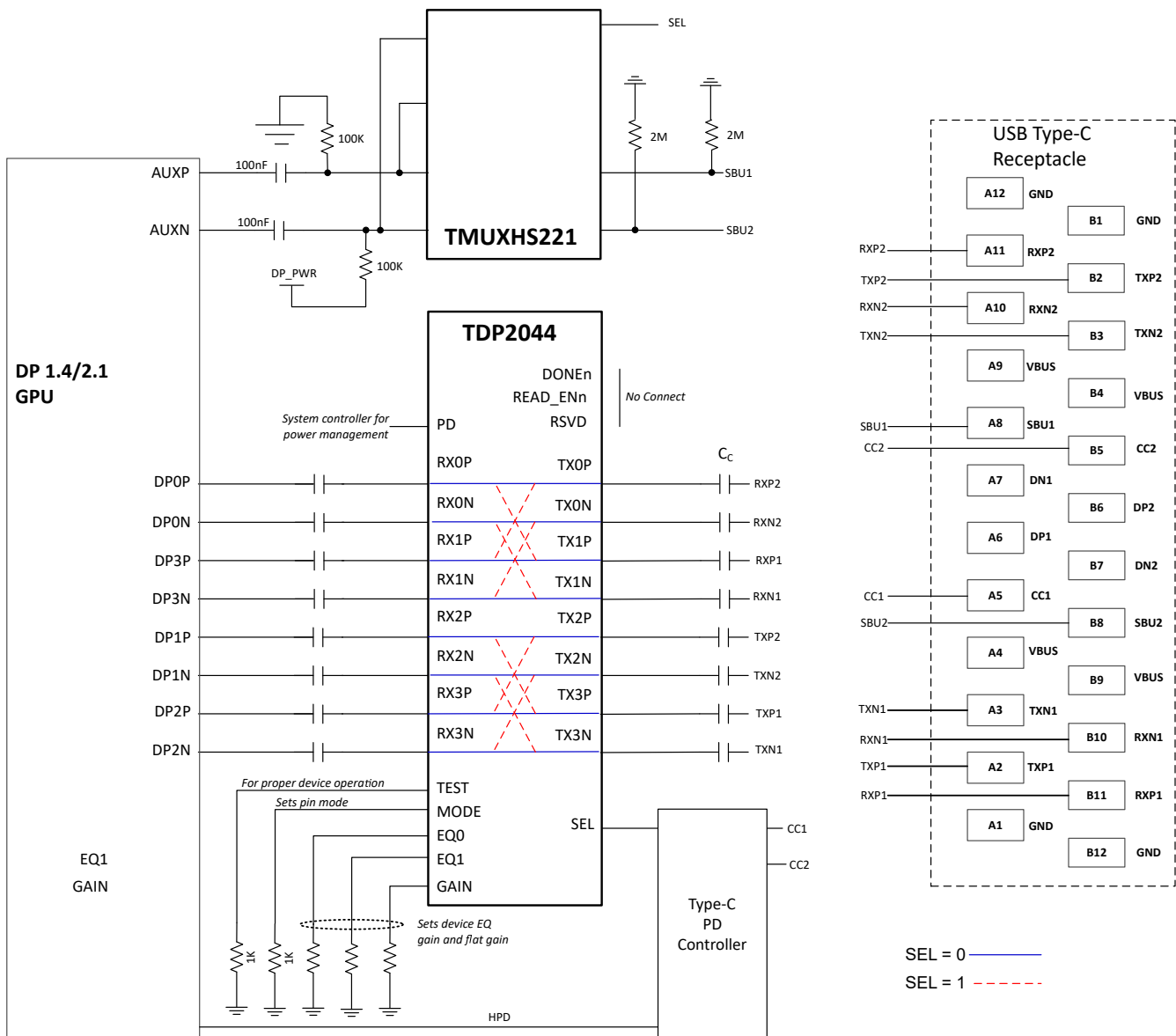
図 7-2. Simplified Schematic for USB-C Alternate Mode Source Application
