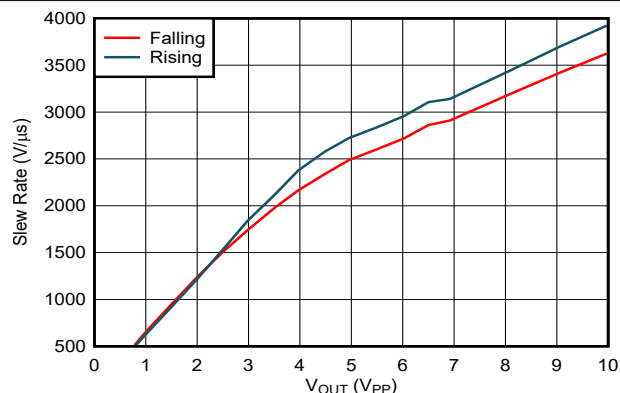
FIG 7-14. Slew Rate vs Output Voltage Step
