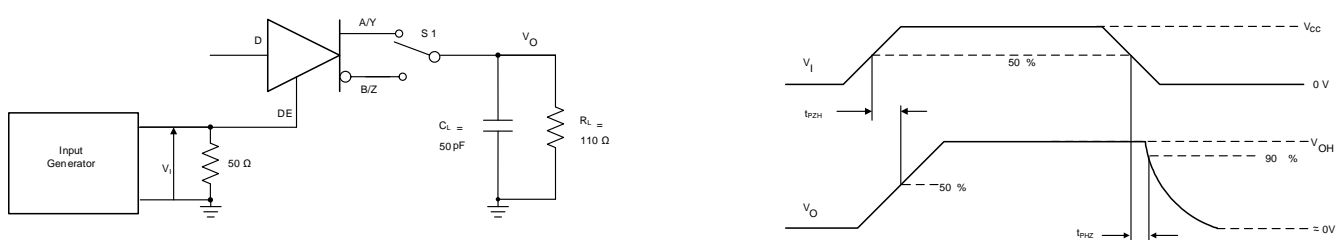
图 23. Measurement of Driver Enable and Disable Times With Active High Output and Pull-Down Load
