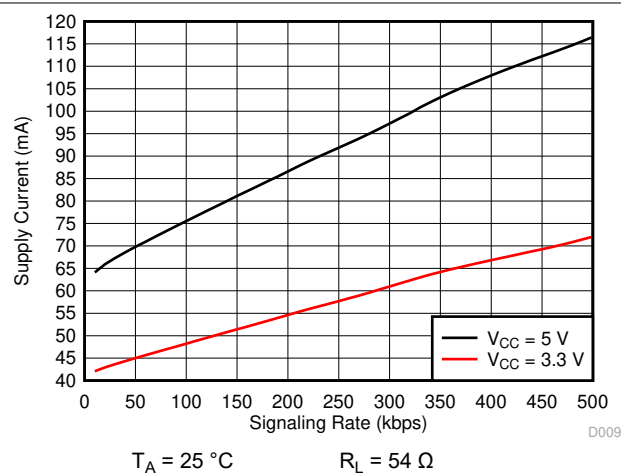
6-6. THVD2410 Supply Current vs Signal Rate
