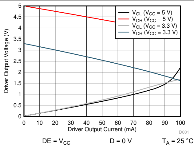
6-1. Driver Output Voltage vs Driver Output Current
