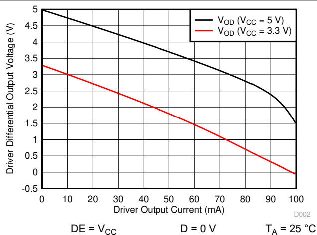
6-2. Driver Differential Output voltage vs Driver Output Current
