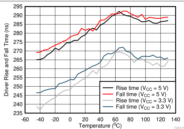
6-4. THVD2410 Driver Rise or Fall Time vs Temperature
