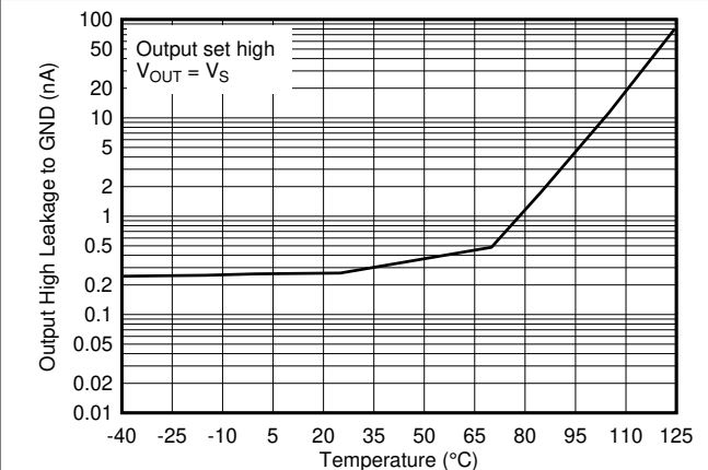
Fig 5-24. Output High Leakage Current vs. Temperature at 36V
