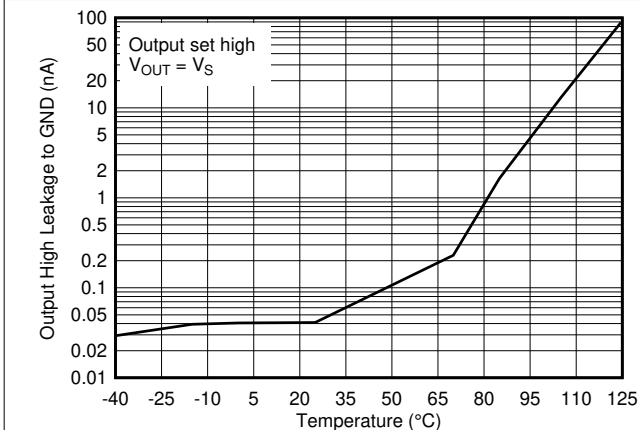
Fig 5-23. Output High Leakage Current vs. Temperature at 5V
