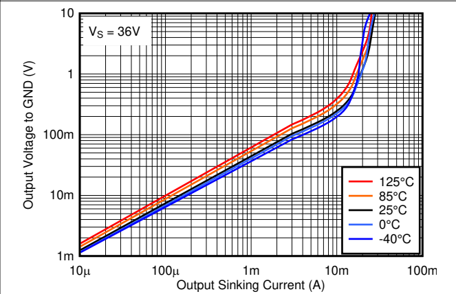
5-22. Output Low Voltage vs. Output Sinking Current at 36V
