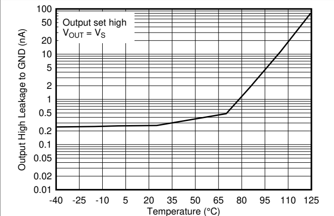
5-24. Output High Leakage Current vs. Temperature at 36V
