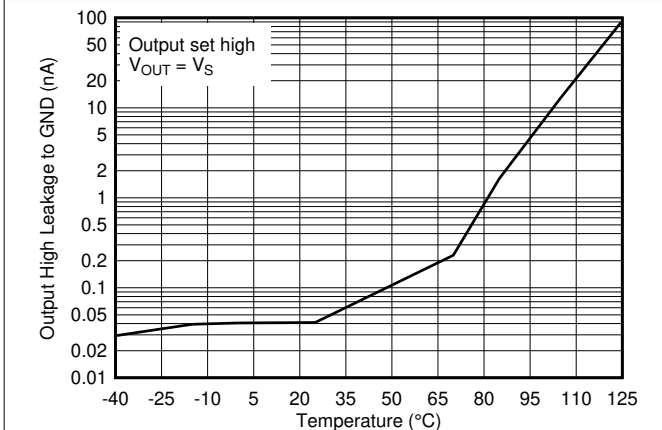
5-23. Output High Leakage Current vs. Temperature at 5V
