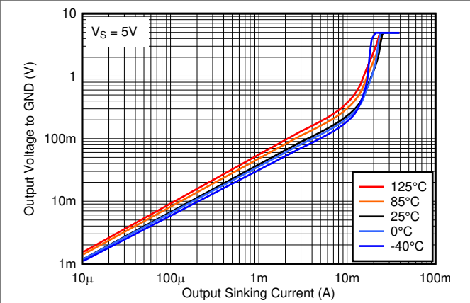
5-20. Output Low Voltage vs. Output Sinking Current at 5V
