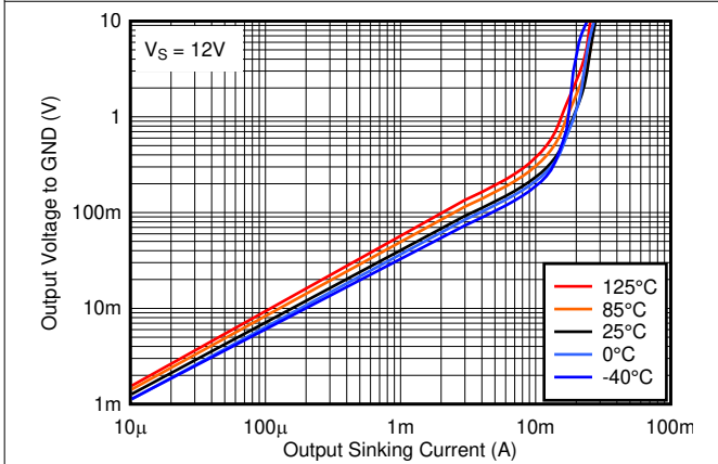
5-21. Output Low Voltage vs. Output Sinking Current at 12V
