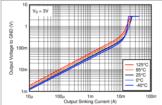
5-19. Output Low Voltage vs. Output Sinking Current at 3V
