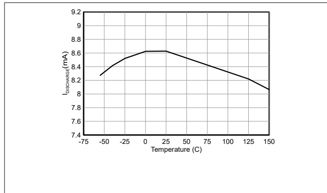
図 5-1. Oscillator Discharge Current vs Temperature for V_{IN} = 15\text{ V} and V_{OSC} = 2\text{ V}
