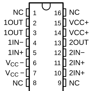
TLE2142 PW PACKAGE (TOP VIEW)
