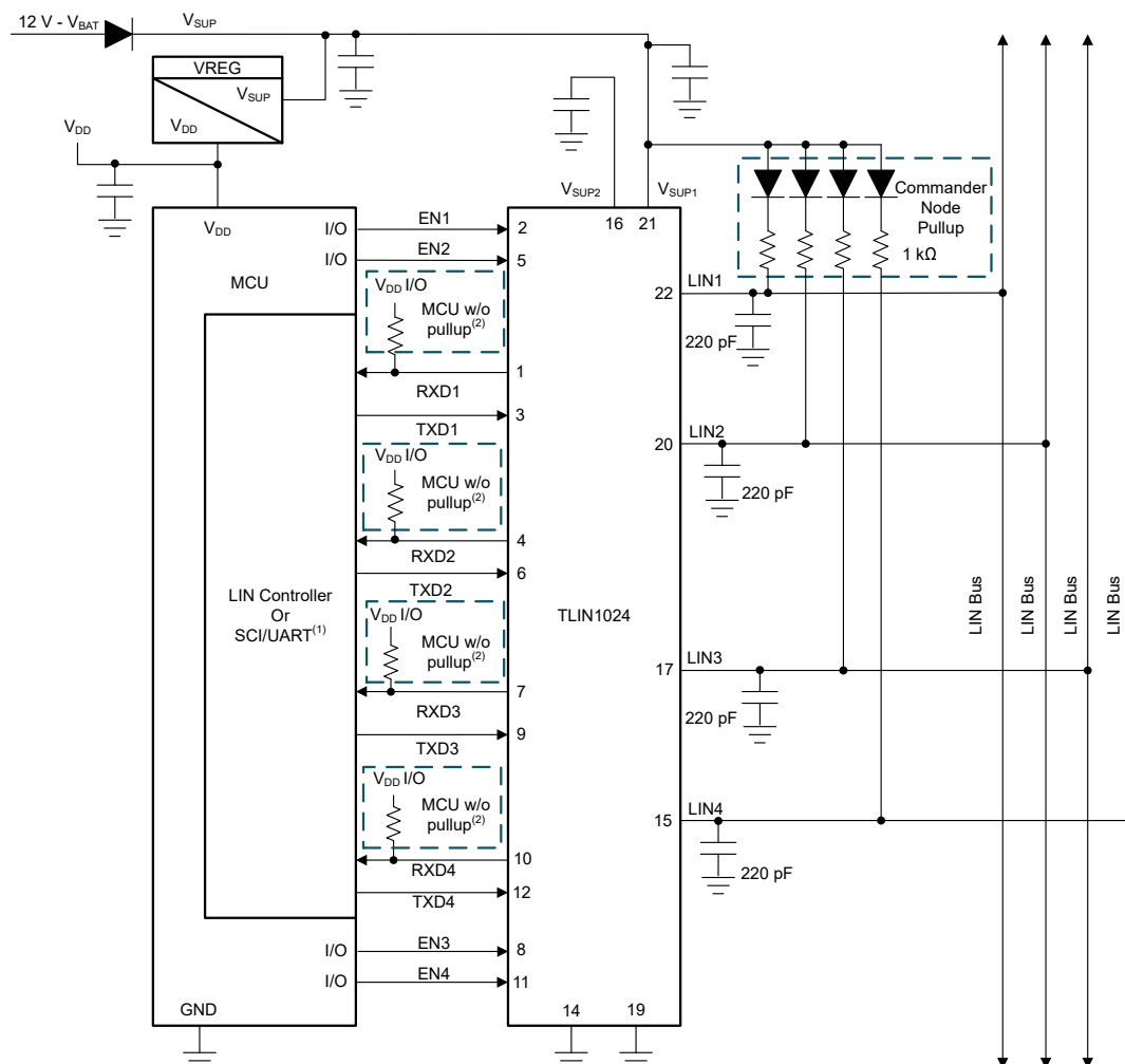
8-1. Typical LIN Bus
