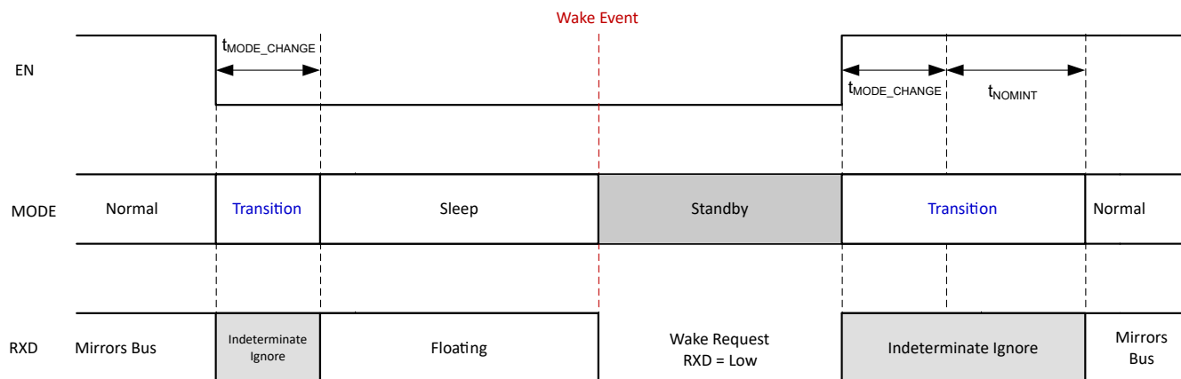
7-15. Mode Transitions
