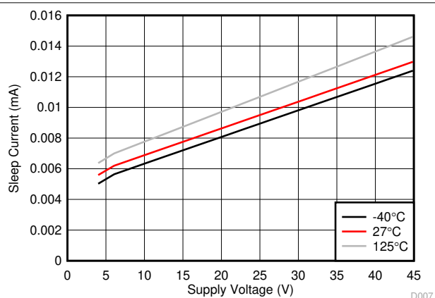
FIG 6-7. Sleep Current vs V_{SUP} and Temperature
