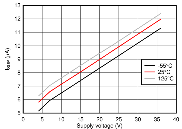
7-6. Standby Recessive I_{SUP} vs V_{SUP} and Temperature
