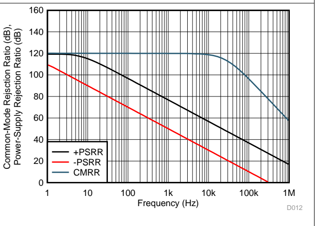
Fig 6. CMRR and PSRR vs Frequency (Referred-to-Input)
