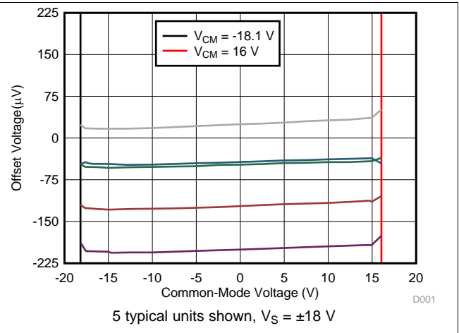
Fig 2. Offset Voltage vs Common-Mode Voltage
