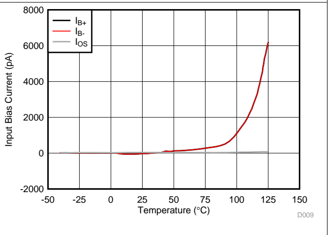
Fig 4. Input Bias Current vs Temperature
