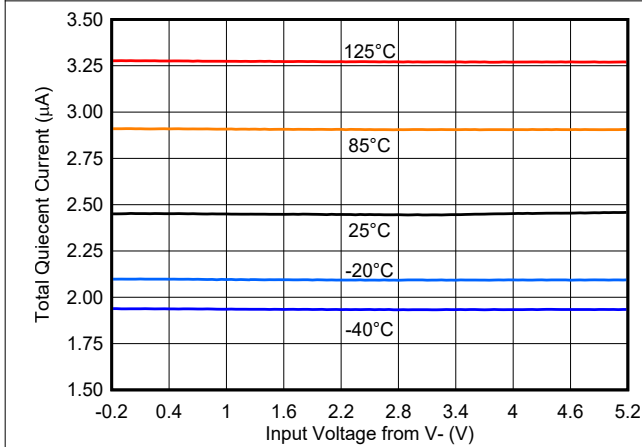
8-11. Supply Current vs. Common Mode - 5V
