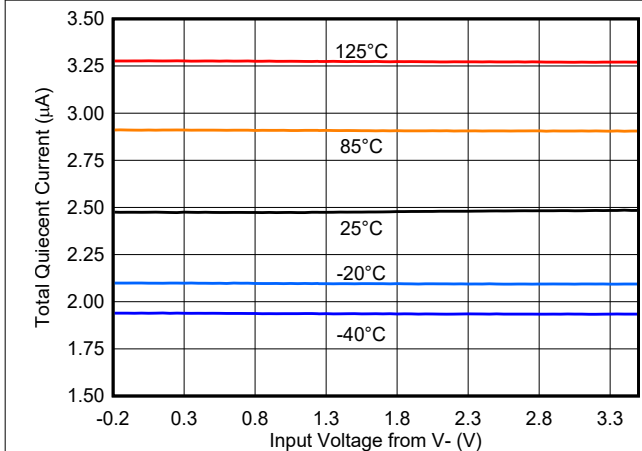
8-9. Supply Current vs. Common Mode - 3.3V
