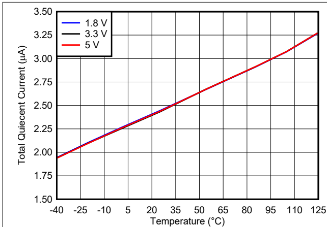
8-7. Supply Current vs. Temperature
