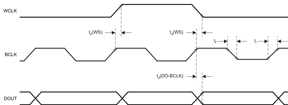
図 2. DSP Timing in Master Mode
