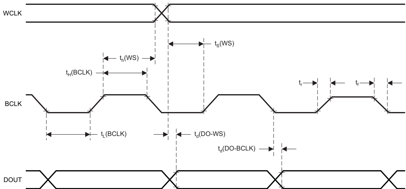
図 3. I²S, LJF, RJF Timing in Slave Mode
