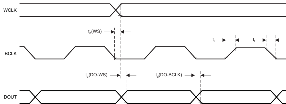
図 1. I²S, LJF, RJF Timing in Master Mode
