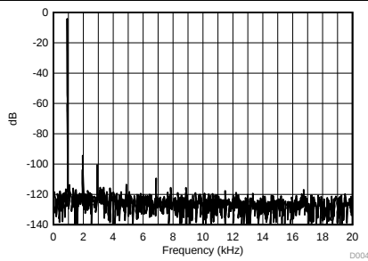
FIG 139. Line Input to ADC FFT Plot
