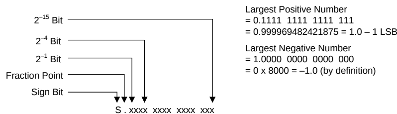
図 39. 2s-Complement Coefficient Format
