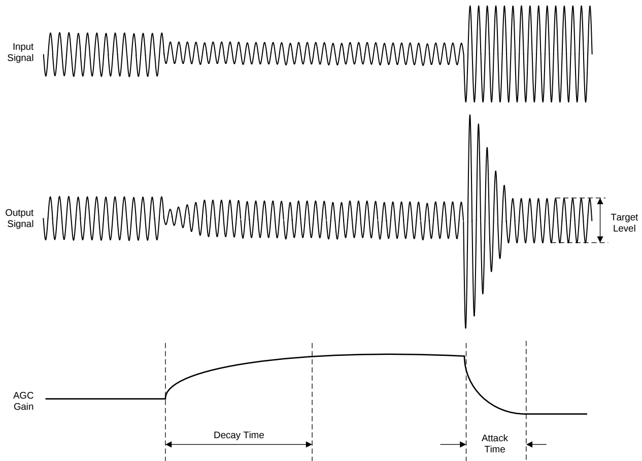
図 28. AGC Characteristics
