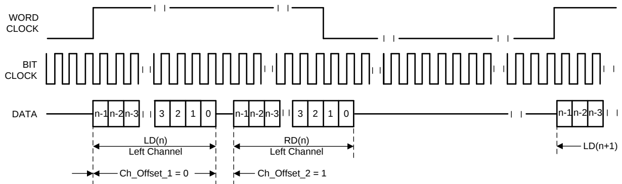
FIG 17. Left-Justified Mode, Time-Based-Slot Mode Enabled, Ch_Offset_1 = 0, Ch_Offset_2 = 1
