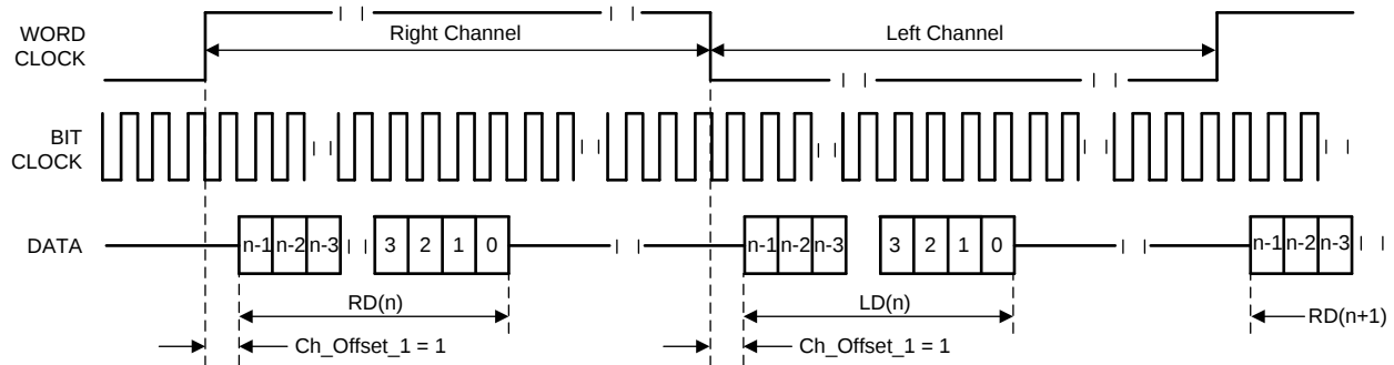
FIG 16. Left-Justified Mode With Ch_Offset_1 = 1, Channel Swapping Enabled
