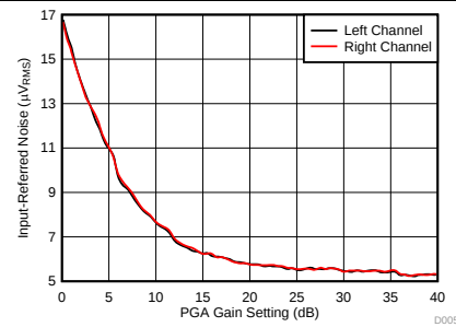
FIG 140. Input-Referred Noise vs PGA Gain
