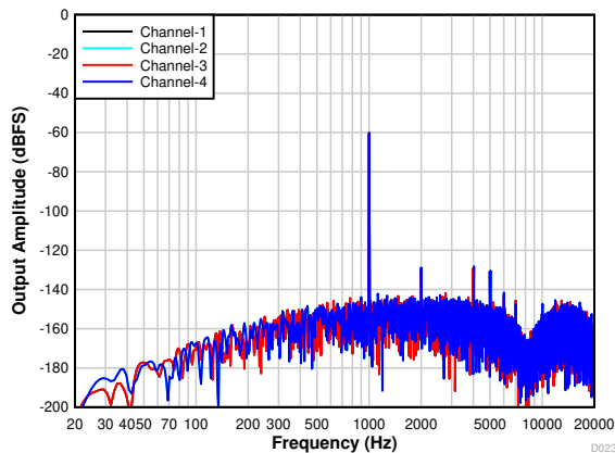
7-26. PDM Input FFT With a -60-dBr Input
