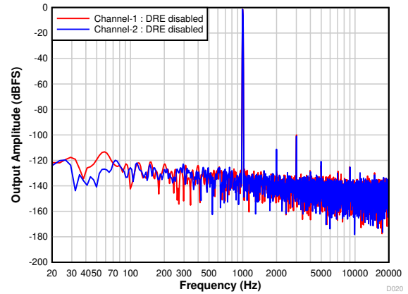
7-23. FFT With a -1-dBr Input With DRE Disabled
