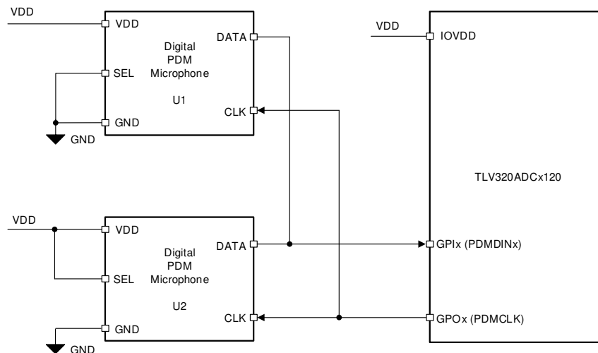
Figure 8-64. Digital PDM Microphones Connection Diagram for the TLV320ADC5120
