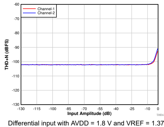
7-9. THD+N vs Input Amplitude With DRE Disabled
