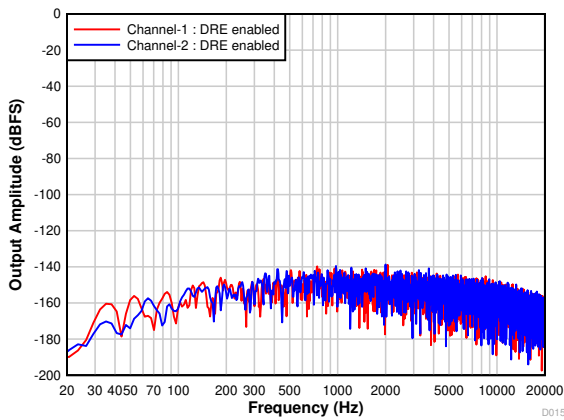
7-18. FFT With Idle Input With DRE Enabled
