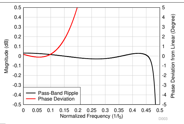
Figure 8-60. Ultra-Low-Latency Decimation Filter Pass-Band Ripple and Phase Deviation
