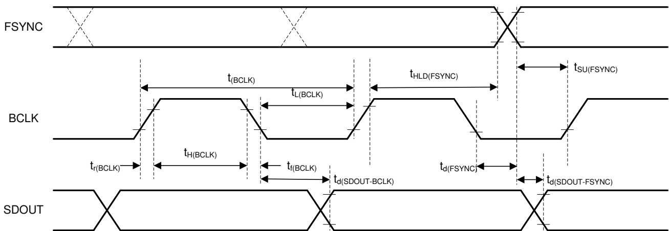
7-2. TDM (With BCLK_POL = 1), I 2 S, and LJ Interface Timing Diagram
