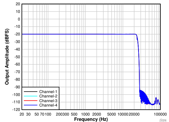
7-27. PDM Input Frequency Response With a -20-dBr Input
