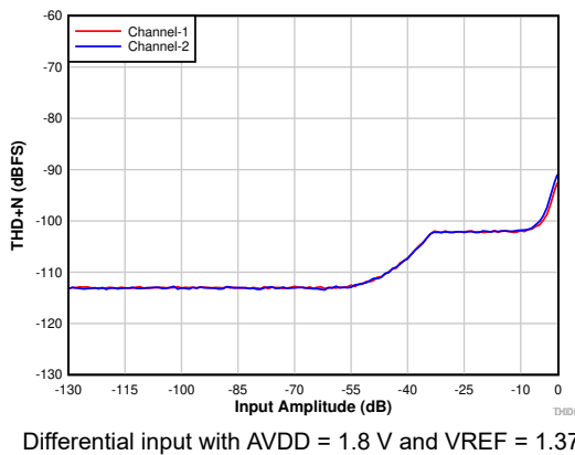
7-8. THD+N vs Input Amplitude With DRE Enabled
