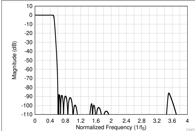
Figure 8-57. Ultra-Low-Latency Decimation Filter Magnitude Response
