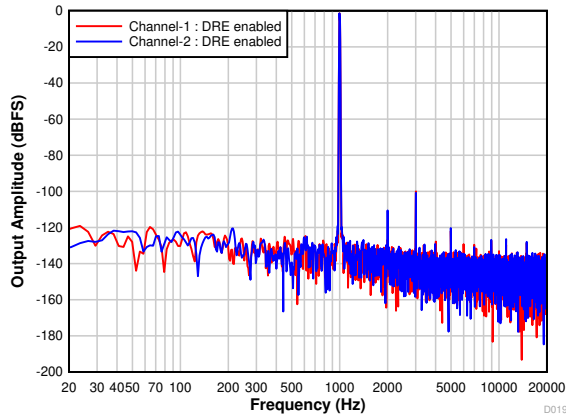
7-22. FFT With a -1-dBr Input With DRE Enabled
