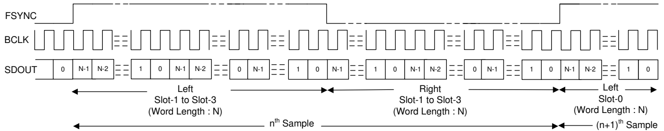
8-11. LJ Protocol Timing (No Idle BCLK Cycles, TX_OFFSET = 0)
