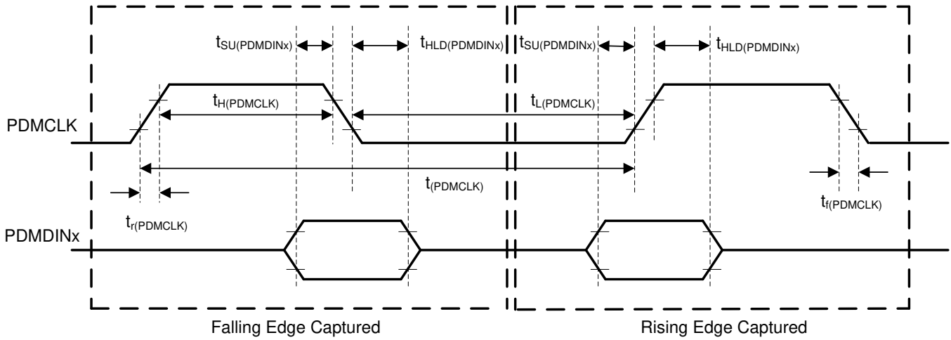
7-3. PDM Digital Microphone Interface Timing Diagram
