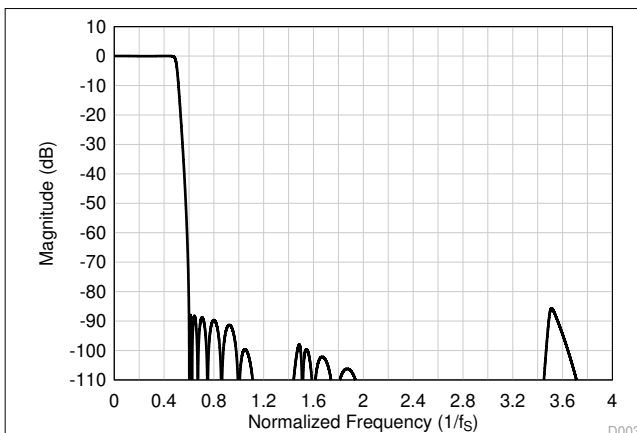
Figure 8-59. Ultra-Low-Latency Decimation Filter Magnitude Response
