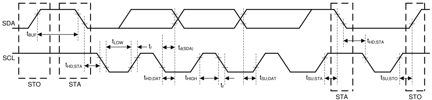
7-1. I 2 C Interface Timing Diagram
