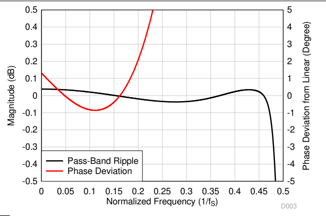
Figure 8-58. Ultra-Low-Latency Decimation Filter Pass-Band Ripple and Phase Deviation
