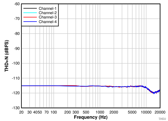
7-25. PDM Input THD+N vs Input Frequency With a -20-dBr Input
