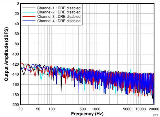
FIG 18. FFT With Idle Input With DRE Disabled
