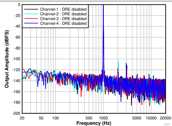
FIG 20. FFT With a -60\text{-dBr} Input With DRE Disabled
