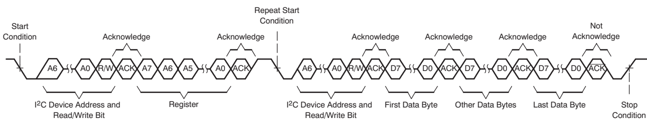
Figure 92. I 2 C Multiple-Byte Read Transfer
