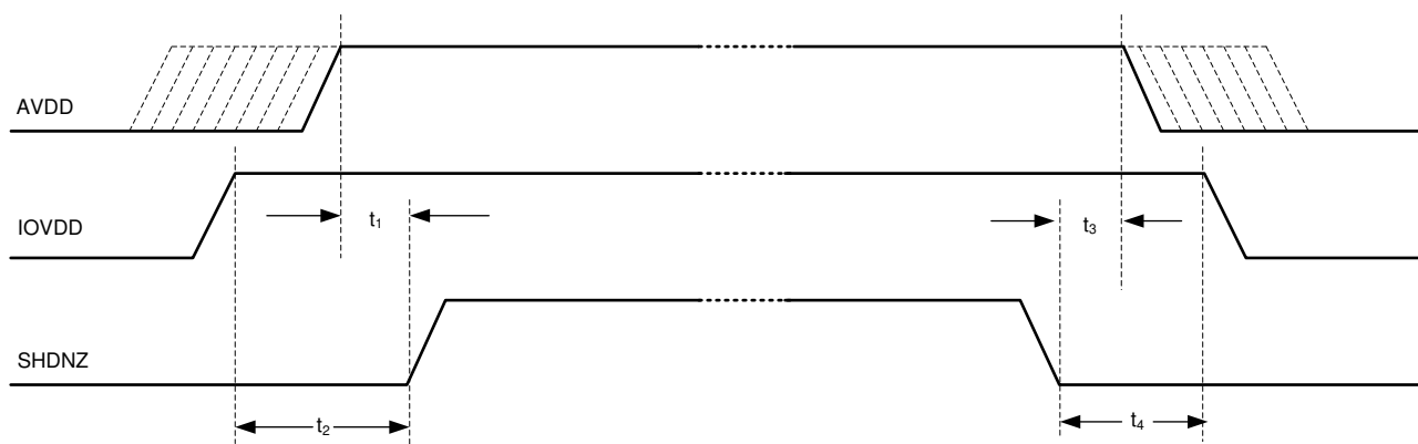
Figure 178. Power-Supply Sequencing Requirement Timing Diagram
