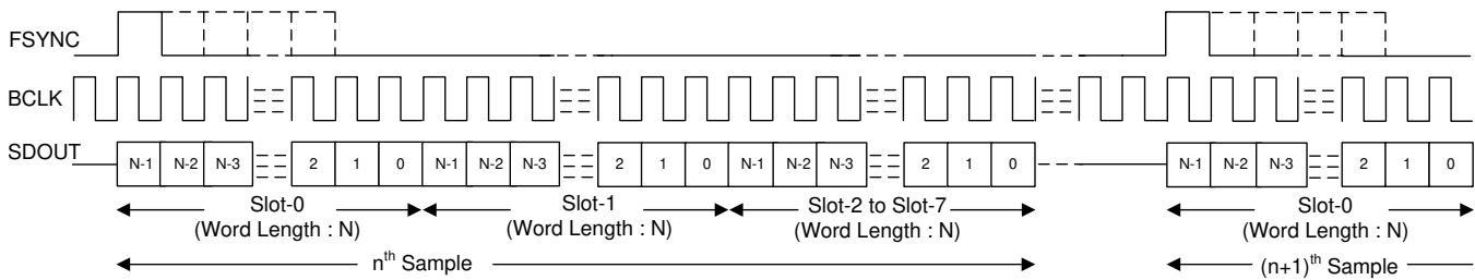
図 23. TDM Mode Standard Protocol Timing (TX_OFFSET = 0)
