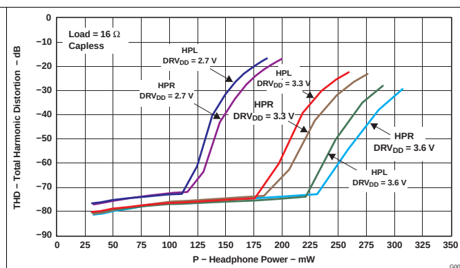
Figure 35. THD vs Headphone Power, Capless
