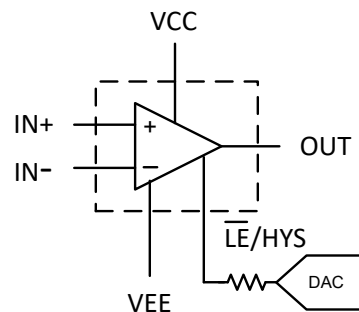
図 7-2. Adjustable Hysteresis using External Voltage
