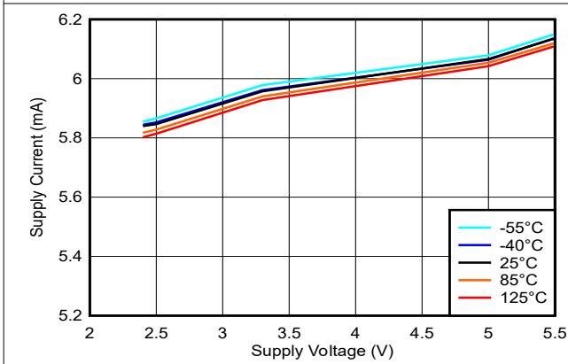
5-23. Supply Current vs. Voltage (Output Low)
