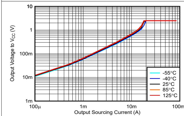
5-17. Output Voltage vs. Output Sourcing Current, 2.5V
