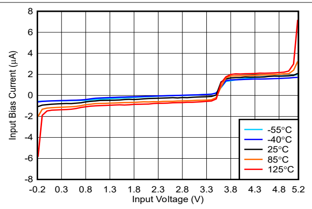
5-16. Bias Current vs. Input Voltage, 5V
