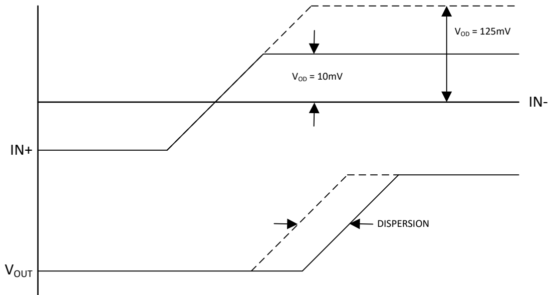
図 5-2. Overdrive Dispersion
