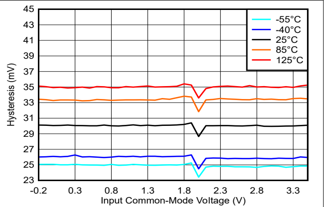
图 5-8. Hysteresis vs. Common-Mode, 3.3V
