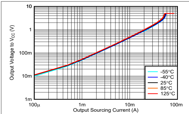
5-21. Output Voltage vs. Output Sourcing Current, 5V
