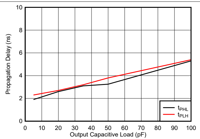
5-34. Propagation Delay vs. Load Capacitance, 5V
