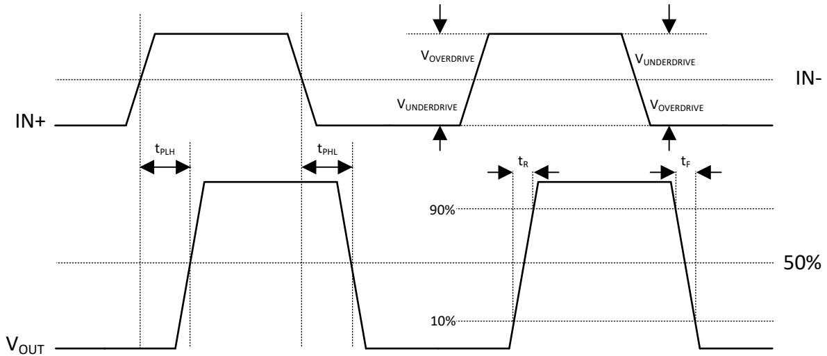
図 5-1. General Timing Diagram
