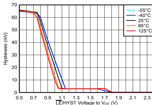
図 7-4. Hysteresis vs. V_{\text{HYS}} at V_{\text{CC}} = 5\text{V}
