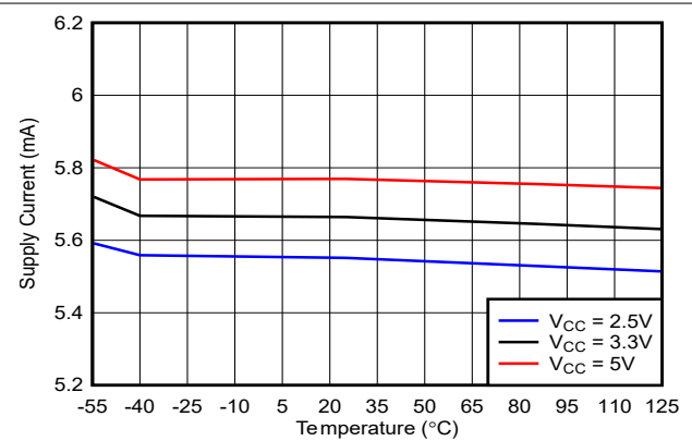
5-26. Supply Current vs. Temp (Output High)
