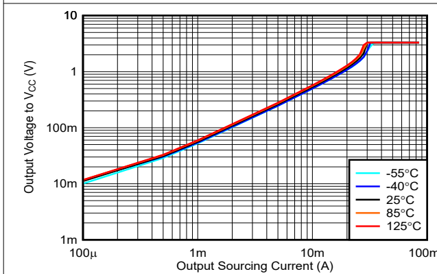
5-19. Output Voltage vs. Output Sourcing Current, 3.3V
