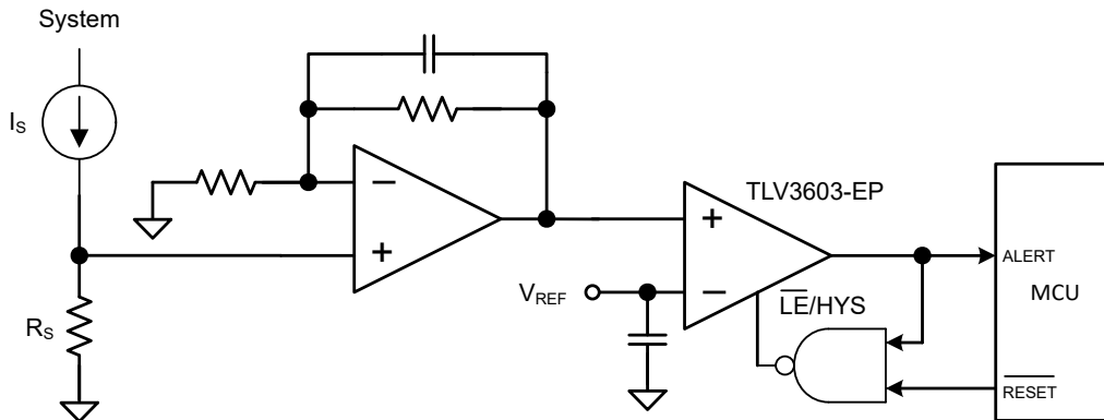
图 7-11. Over-Current Latched Output Circuit
