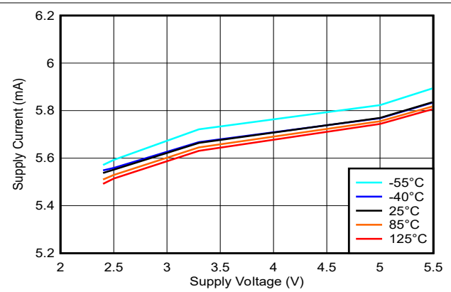
5-24. Supply Current vs. Voltage (Output High)
