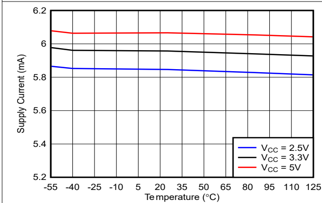
5-25. Supply Current vs. Temp (Output Low)
