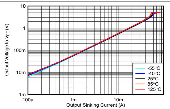
5-22. Output Voltage vs. Output Sinking Current, 5V
