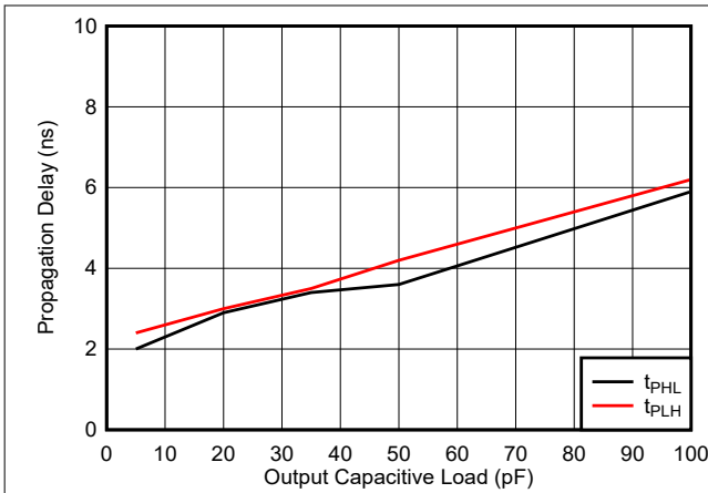
5-33. Propagation Delay vs. Load Capacitance, 3.3V
