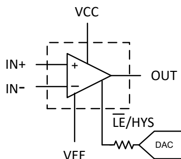
図 7-2. Adjustable Hysteresis using External Voltage
