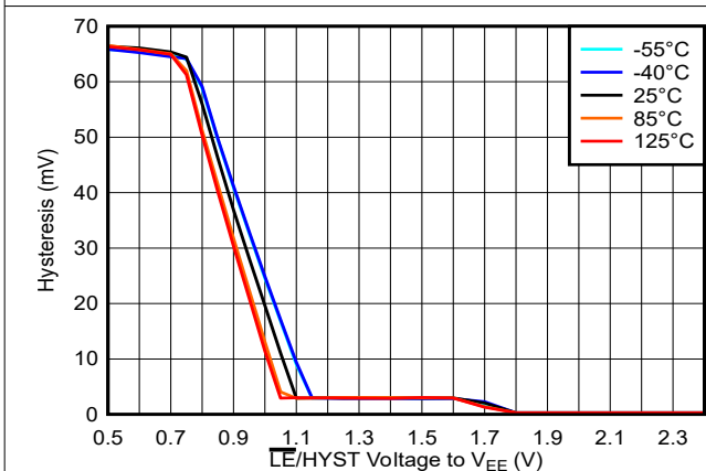
5-37. Hysteresis Voltage vs. \overline{LE}/HYST Voltage, 3.3V
