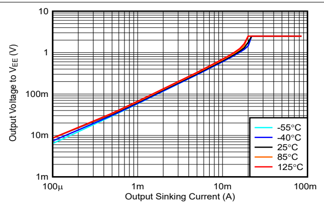
5-18. Output Voltage vs. Output Sinking Current, 2.5V
