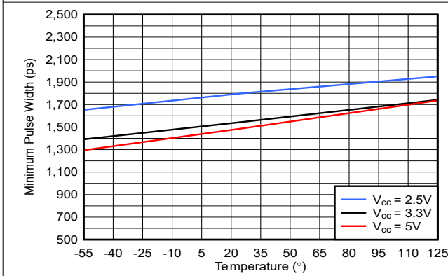
5-35. Minimum Pulse Width vs. Temperature
