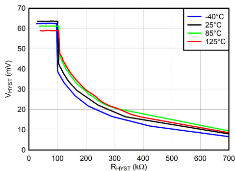
図 7-7. V_{HYST} vs. R_{HYST} at 5V curve
