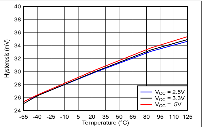
图 5-4. Hysteresis vs. Temperature
