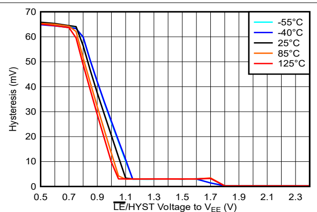
5-38. Hysteresis Voltage vs. \overline{LE}/HYST Voltage, 5V
