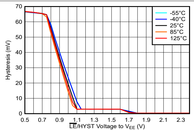
5-36. Hysteresis Voltage vs. \overline{LE}/HYST Voltage, 2.5V
