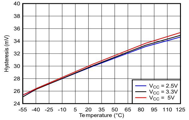
图 5-4. Hysteresis vs. Temperature
