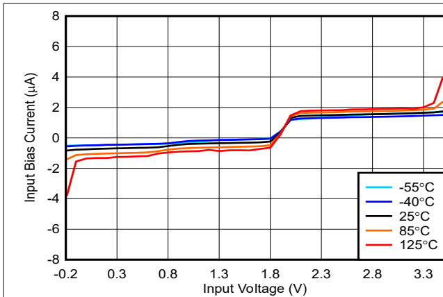
5-15. Bias Current vs. Input Voltage, 3.3V
