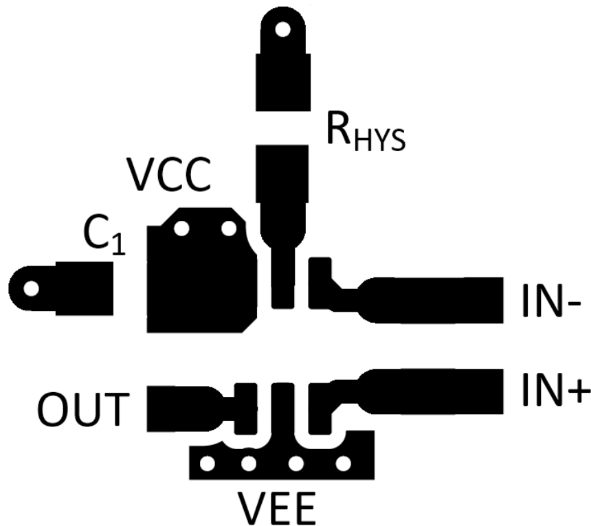
☒ 9-1. TLV3603-EP Layout Example
