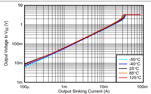
5-20. Output Voltage vs. Output Sinking Current, 3.3V
