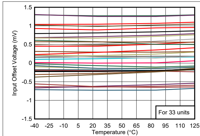
Figure 6-3. Offset vs. Temperature
