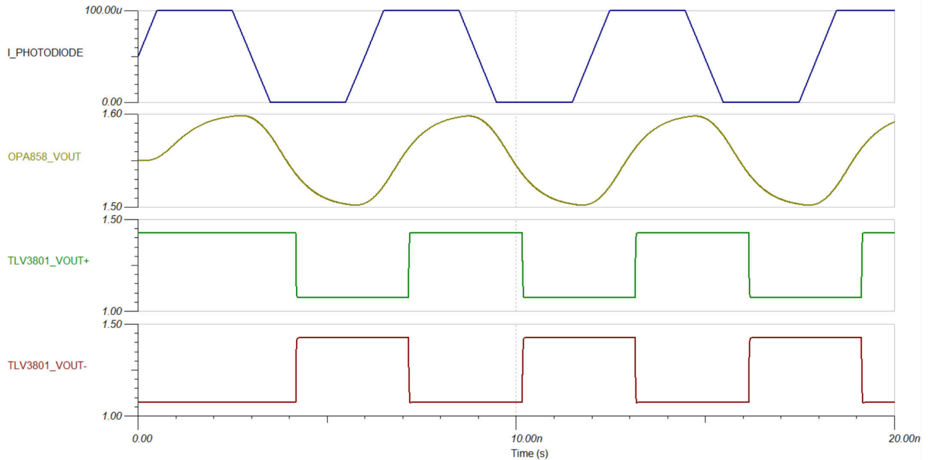
図 8-2. Optical Receiver Output Waveforms
