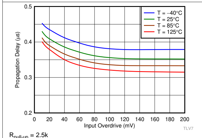
Figure 7. TLV7021 Propagation Delay (L-H) vs. Input Overdrive
