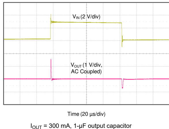
6-12. Line Transient
