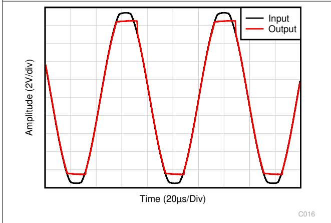
6-29. No Phase Reversal
