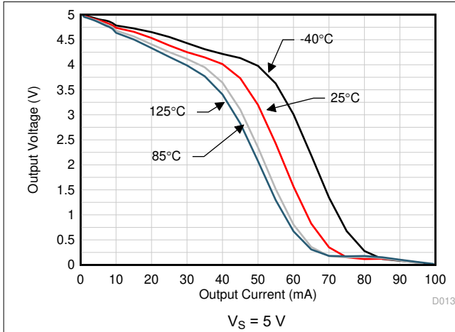
Figure 6-13. Output Voltage Swing vs Output Current (Sourcing)
