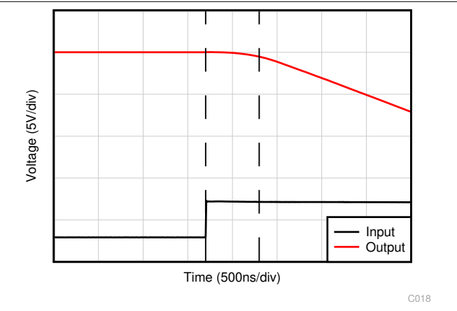
6-30. Positive Overload Recovery
