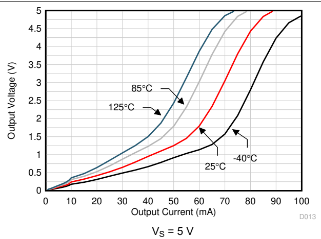
Figure 6-14. Output Voltage Swing vs Output Current (Sinking)
