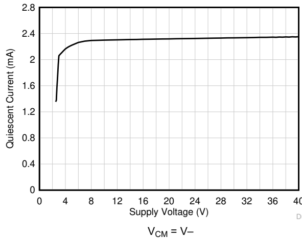
6-22. Quiescent Current vs Supply Voltage
