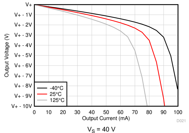
6-12. Output Voltage Swing vs Output Current (Sourcing)
