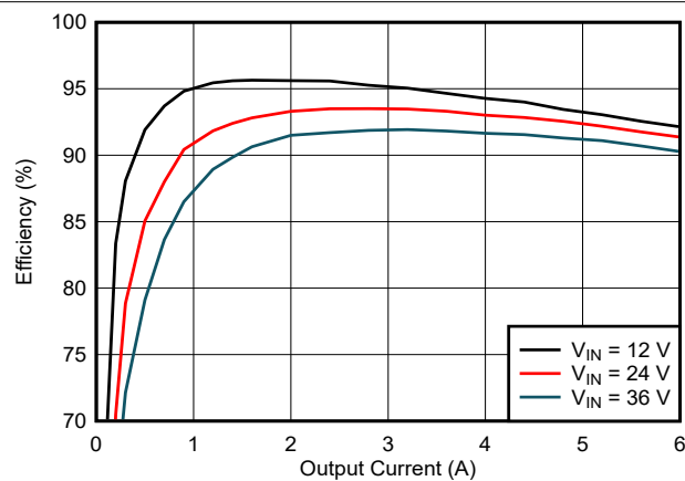
图 9-2. Efficiency
