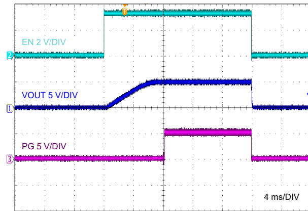
图 9-5. Enable ON and OFF, V_{IN} = 12\text{ V}
