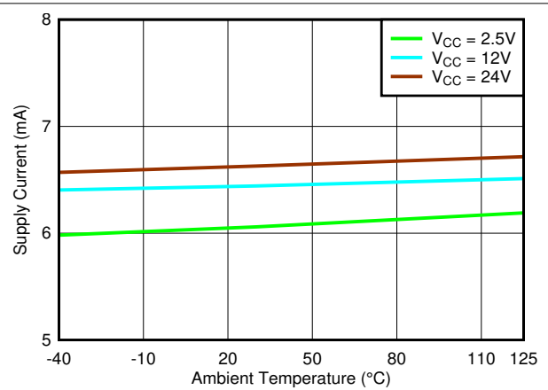
7-76. Supply Current vs. Temperature
