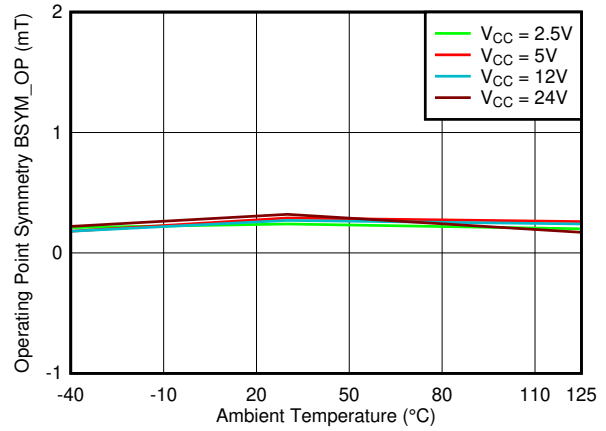
7-30. B_{SYM\_OP(ZY)} vs. Temperature
