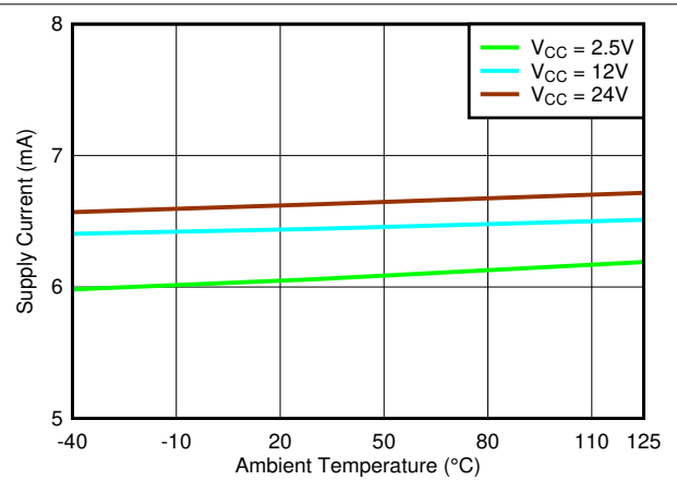
7-76. Supply Current vs. Temperature
