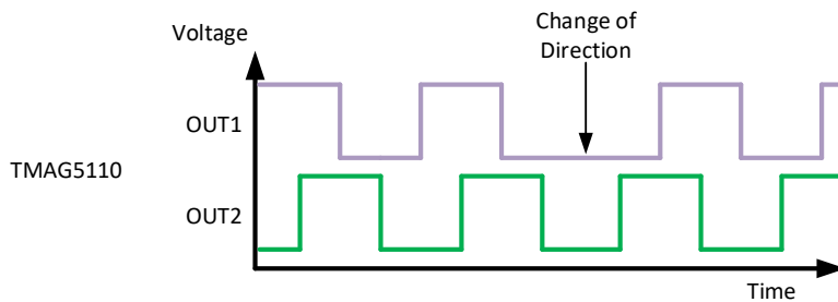
图 9-2. TMAG5110 Output Response
