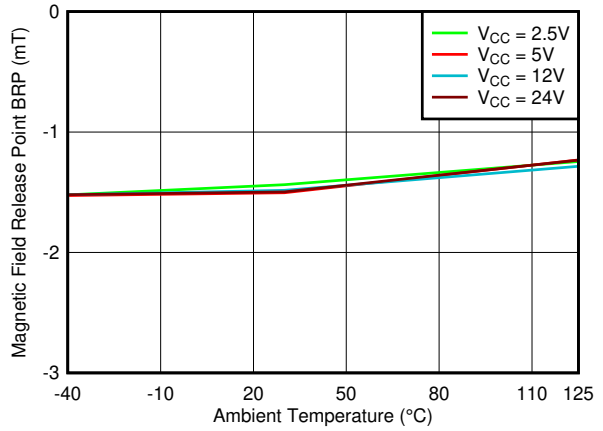
7-16. B RP_Y Threshold vs. Temperature
