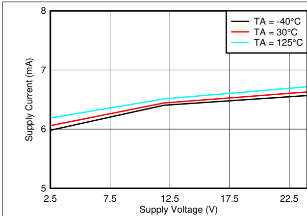
7-75. Supply Current vs. V CC
