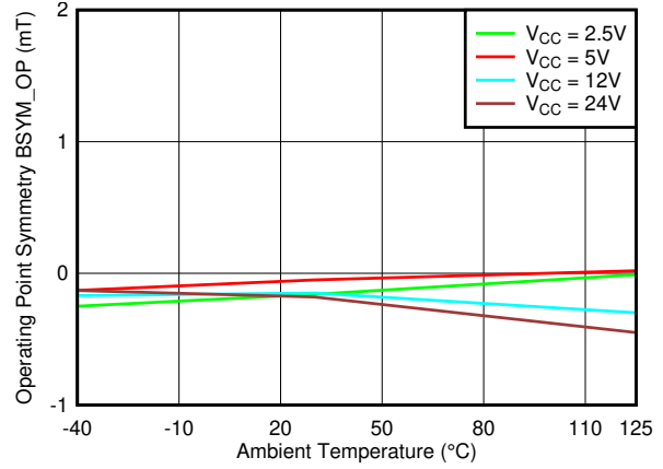
7-26. B_{SYM\_OP(ZX)} vs. Temperature
