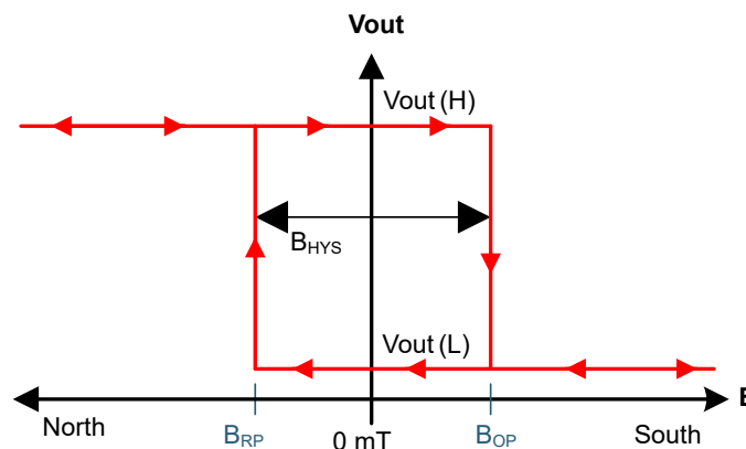
8-2. Latch Functionality
