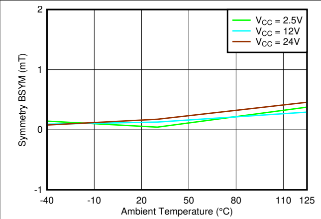
图 7-58. B_{SYM(z)} vs. Temperature
