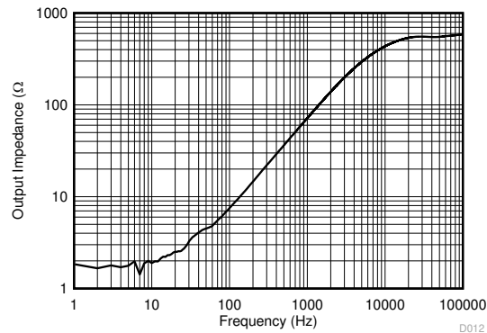
TMP23x-Q1: T_A = 25^\circ\text{C} , V_{DD} = 5\text{ V} , I_{OUT} = 100\ \mu\text{A}
