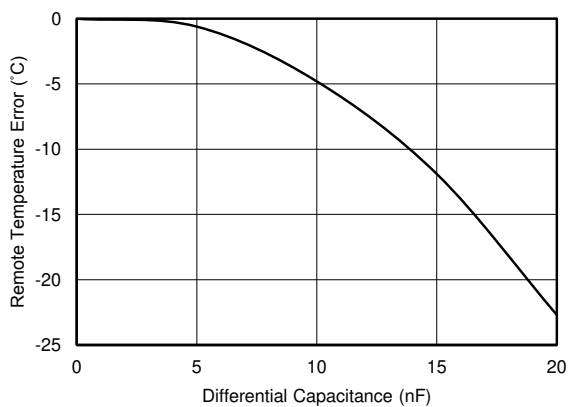
FIG 6-6. Remote Temperature Error vs. Differential Capacitance
