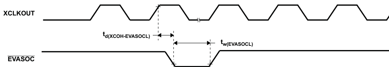
Figure 5-17. EVASOC Timing
