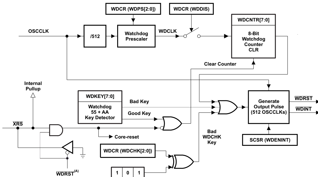
Figure 6-22. Watchdog Module
