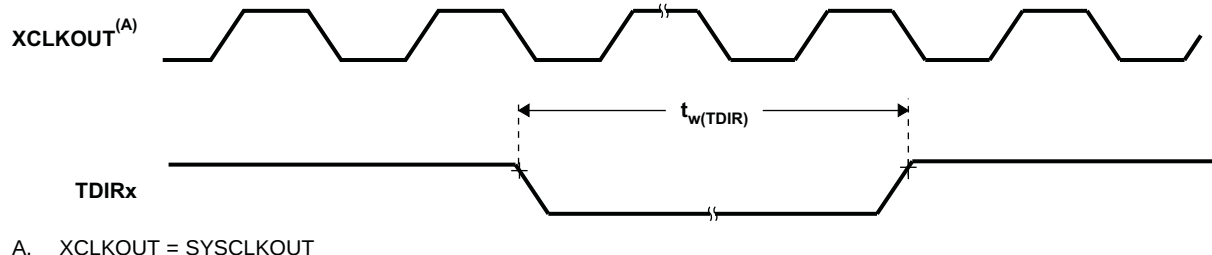
Figure 5-16. TDIRx Timing
