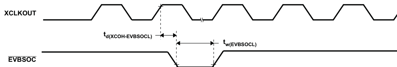
Figure 5-18. EVBSOC Timing
