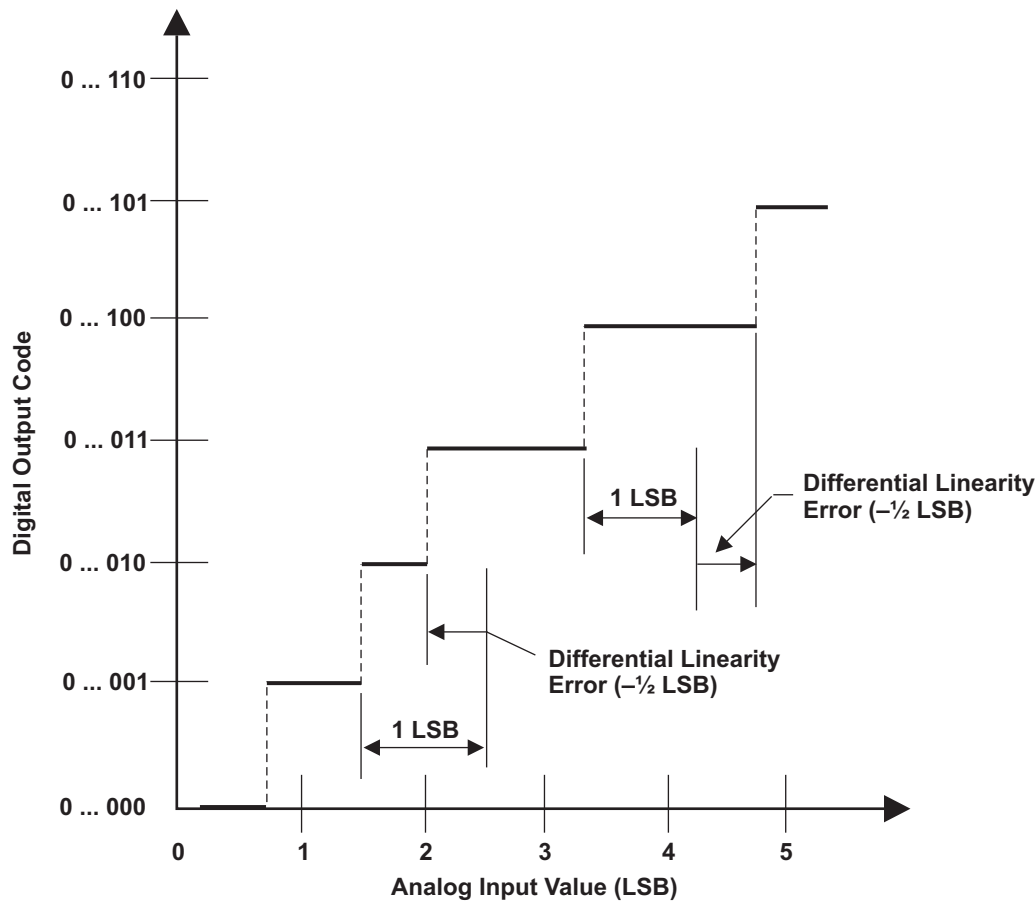
Figure 6-11. Differential Nonlinearity (DNL) Error
