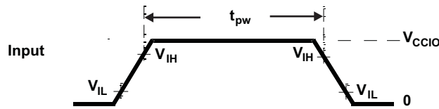
Figure 4-3. TTL-Level Inputs
