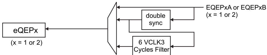
Figure 6-7. eQEPx Input Synchronization Selection Detail
