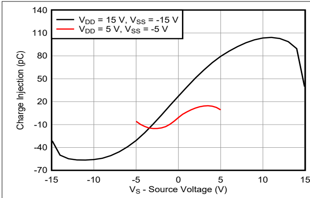
图 5-13. Charge Injection vs Source Voltage – Dual Supply
