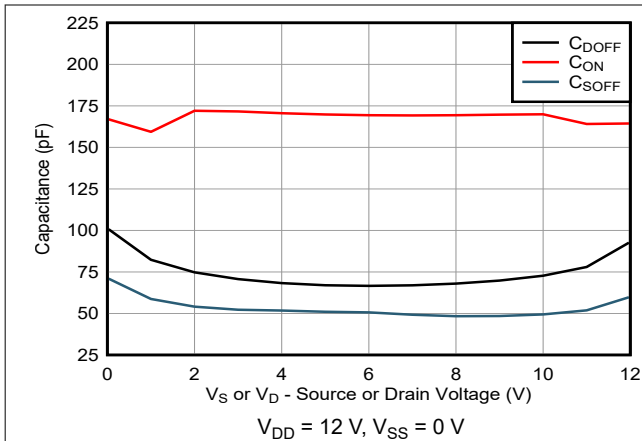
图 5-25. Capacitance vs Source or Drain Voltage
