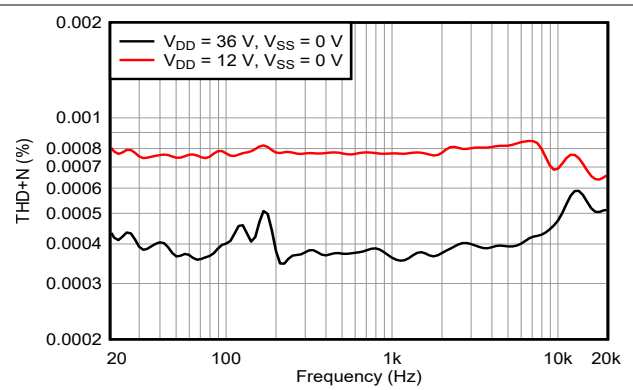
图 5-26. THD+N vs Frequency – Single Supply
