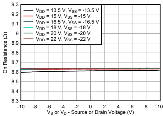
FIG 6-1. On-Resistance vs Source or Drain Voltage
