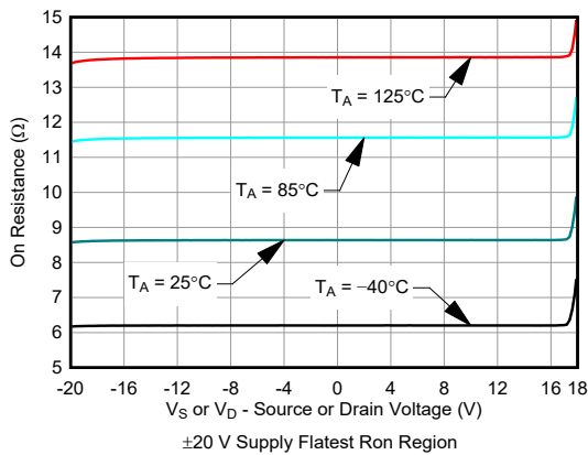
FIG 6-5. On-Resistance vs Source or Drain Voltage
