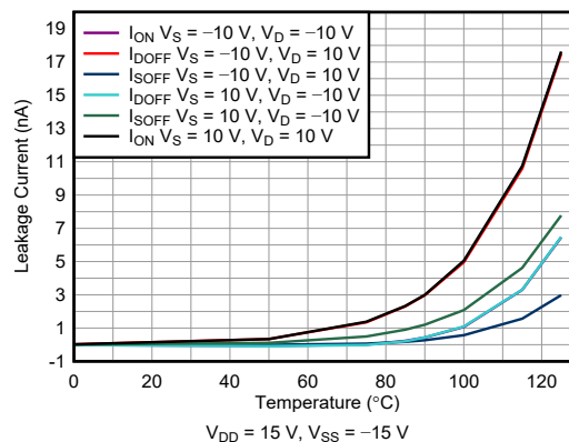
Figure 6-14. Leakage Current vs Temperature
