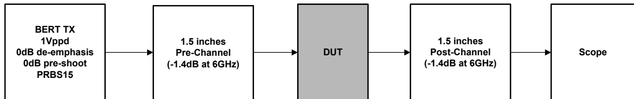
Figure 8-3. Test Setup
