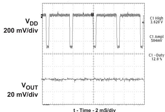
GSM POWER SUPPLY REJECTION vs TIME
