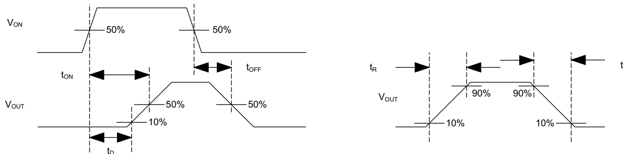
Figure 22. Timing Waveforms
