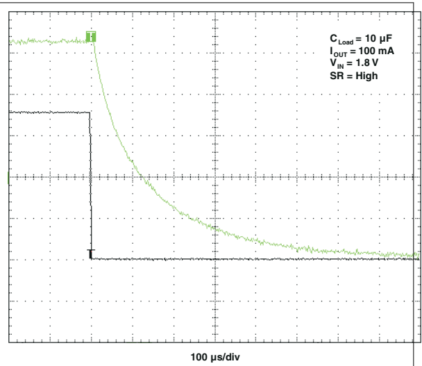
5-17. t_{OFF} Response
