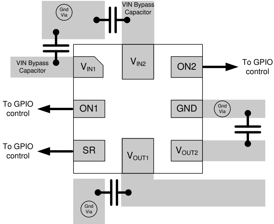
☒ 8-5. RSE Package Layout
