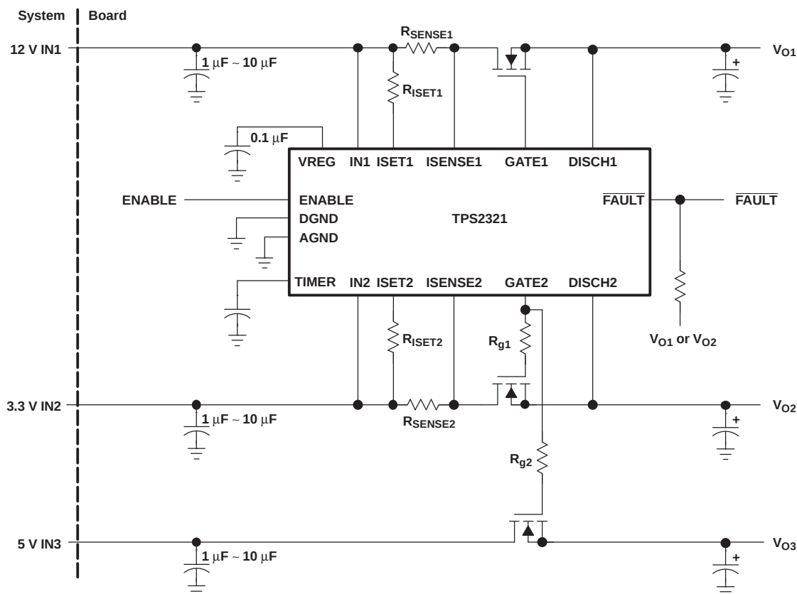
Figure 27. Three-Channel Application
