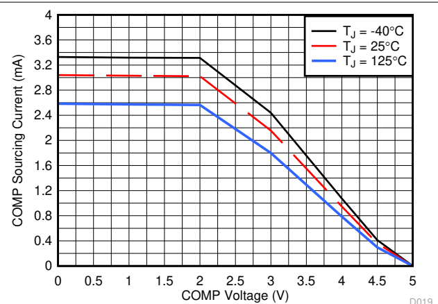
7-16. Error Amplifier Source Current
