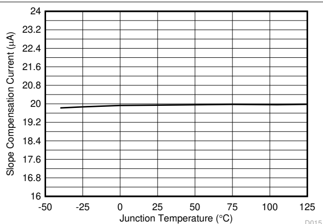
7-14. Current Slope Compensation Current vs Temperature
