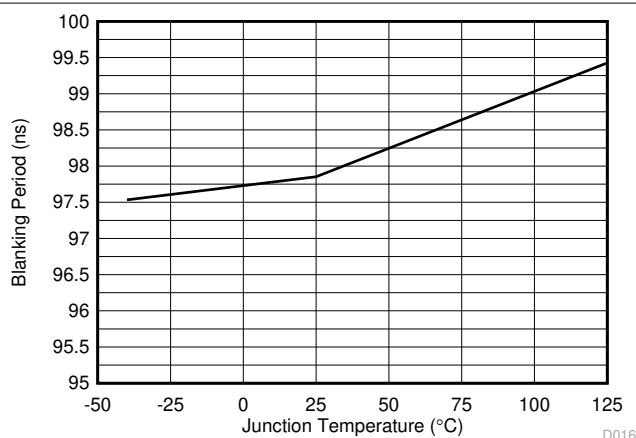
7-15. Blanking Period vs Temperature
