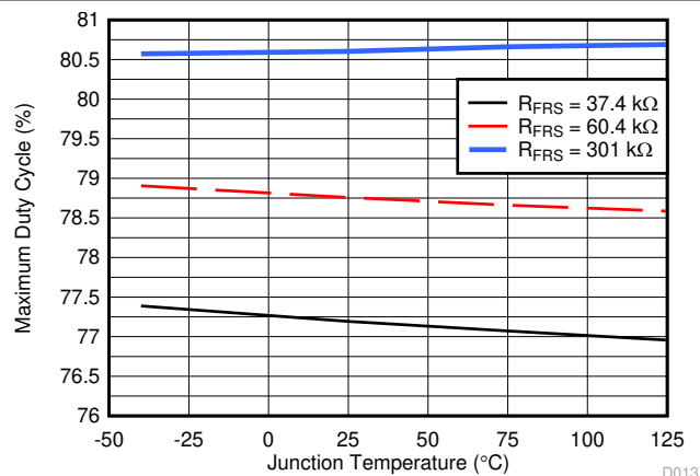
7-12. Maximum Duty Cycle vs Temperature
