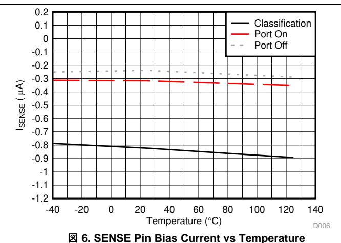
Figure 6. SENSE Pin Bias Current vs Temperature
