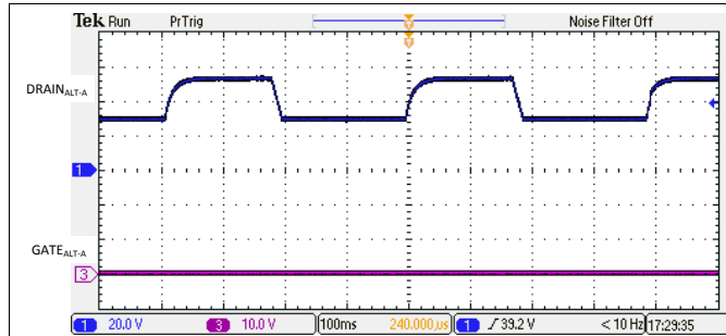
131. 2-Pair Open Circuit Detection Signature
