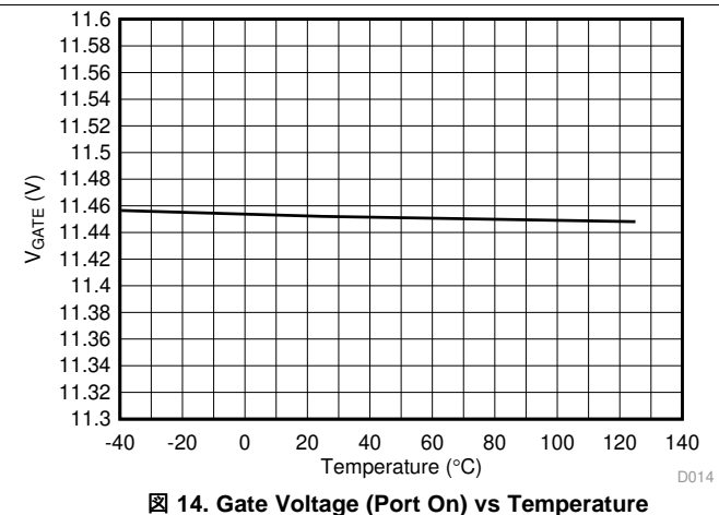
Figure 14. Gate Voltage (Port On) vs Temperature
