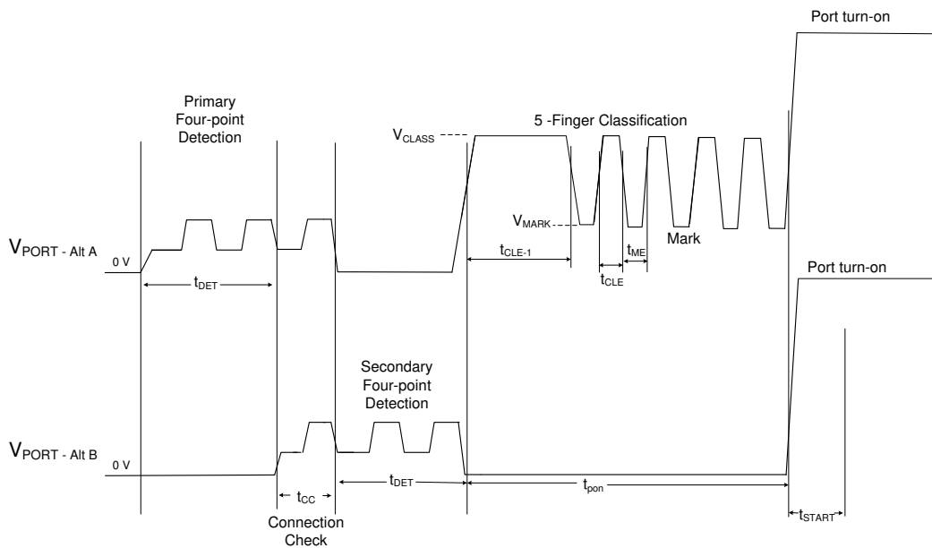
⊠ 36. 4-Pair Single Signature Detection, 5-Event Classification and Turn On
