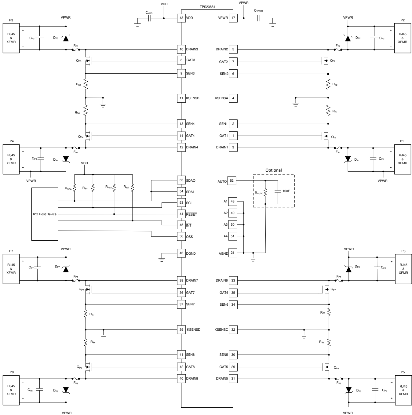
⊠ 122. Eight 2-Pair Port Application
