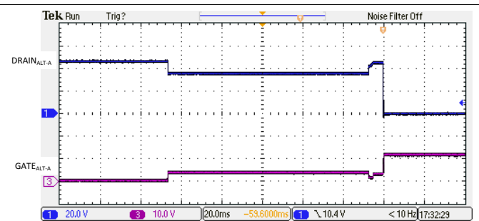
136. 2-Pair 1-Finger Classification and Turn On
