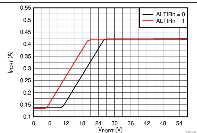
图 28. Inrush Current Foldback vs Port Voltage
