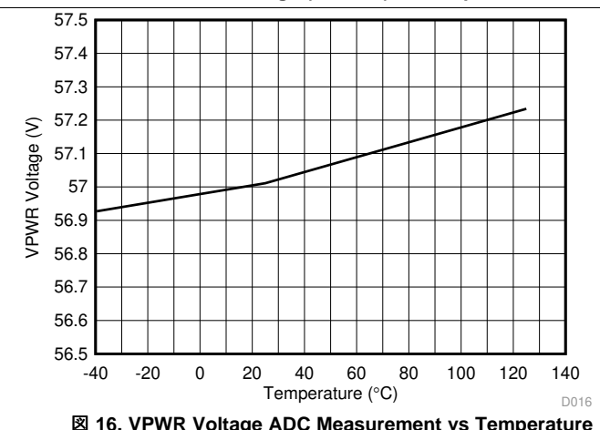
Figure 16. VPWR Voltage ADC Measurement vs Temperature
