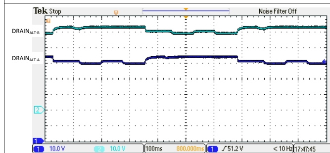
133. 4-Pair Low Resistance (11k \Omega ) Detection Signature
