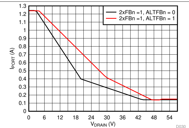
图 30. 2x Mode (2xFBn = 1) Current Foldback vs Drain Voltage
