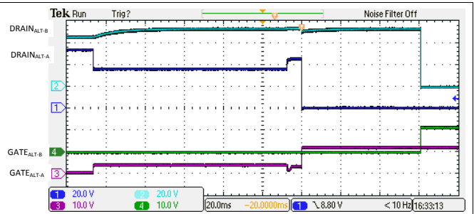
Figure 140. 4-Pair Single Signature Turn On 1-Finger Classification and Turn On
