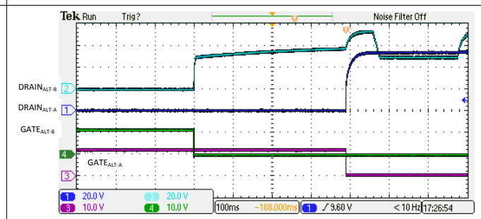
图 130. 4-Pair Single Signature Class 0-4 Disconnect
