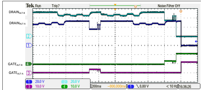
Figure 139. 4-Pair Single Signature Discovery and Turn On from Semi-Auto Mode
