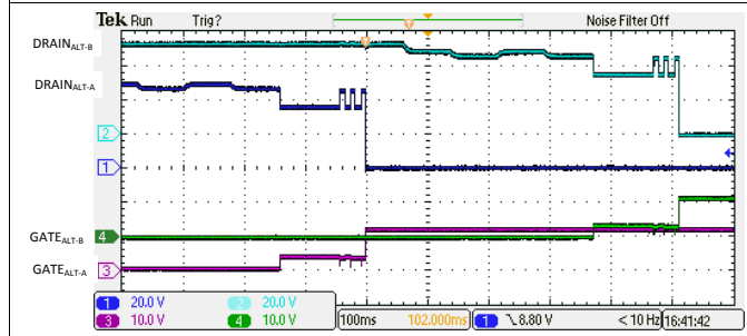
147. 4-Pair Dual Signature 3-Finger Classification and Turn On
