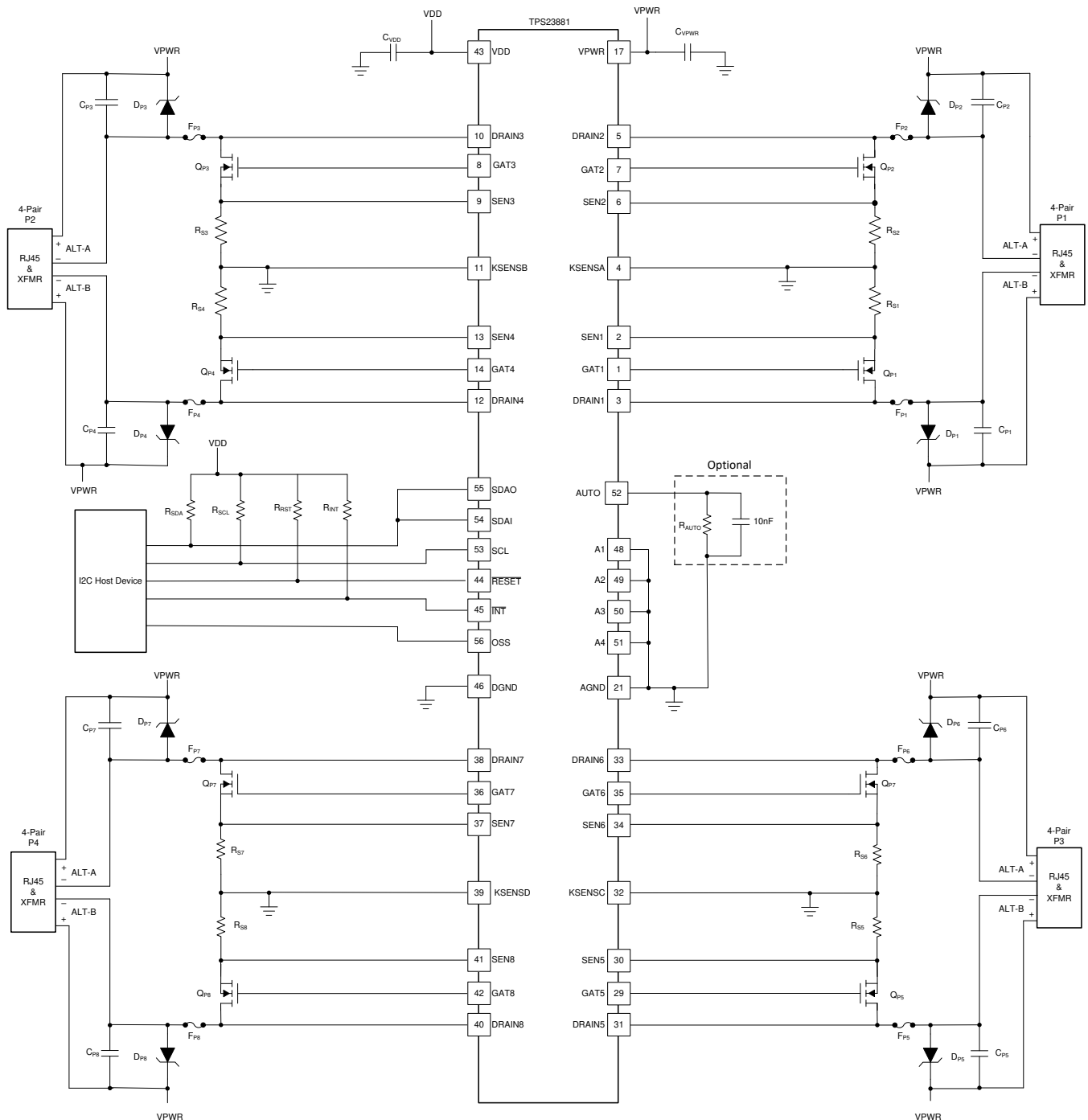
123. Four 4-Pair Port Application
