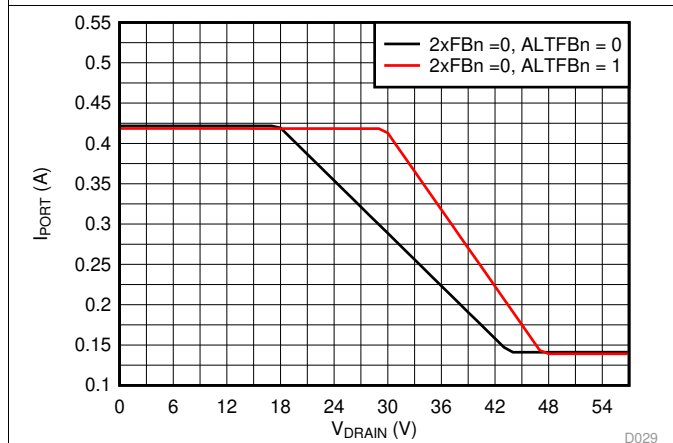
图 29. 1x Mode (2xFBn = 0) Current Foldback vs Drain Voltage
