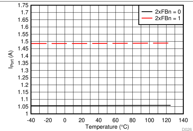
图 26. I_SHORT Threshold vs Temperature
