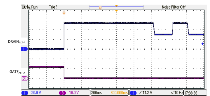
图 126. 2-Pair Backoff due to PCut Fault
