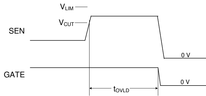
图 32. Overcurrent Fault Timing
