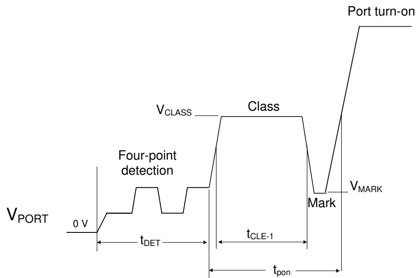
☒ 33. 2-Pair Detection, 1-Event Classification and Turn On
