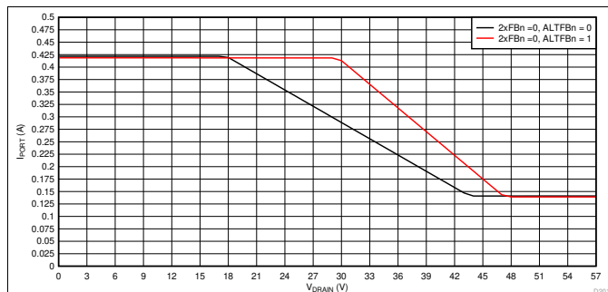
116. 1x Mode (2xFBn = 0) Foldback Curves, I PORT vs V DRAIN
