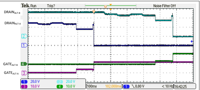
146. 4-Pair Dual Signature 1-Finger Classification and Turn On
