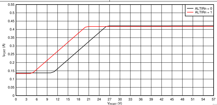
118. Inrush Foldback Curves, I PORT vs V PORT
