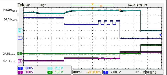
Figure 142. 4-Pair Single Signature 4-Finger Classification and Turn On
