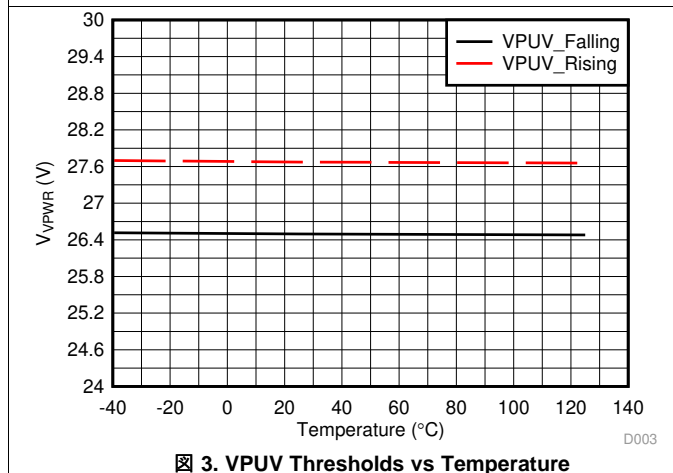
Figure 3. VPUV Thresholds vs Temperature
