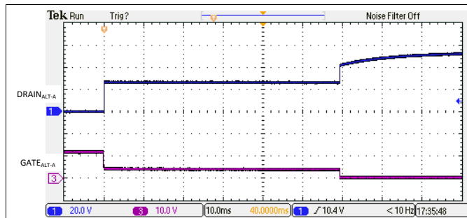
图 125. 2-Pair I_{LIM} Foldback and Turn Off
