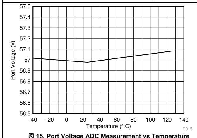
Figure 15. Port Voltage ADC Measurement vs Temperature
