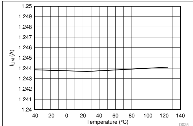
图 25. 2x Mode (2xFBn = 1) Current Limit vs Temperature
