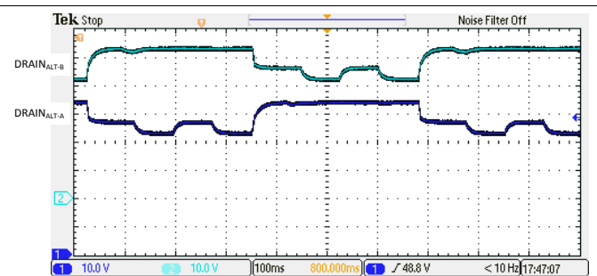
134. 4-Pair High Resistance (36k \Omega ) Detection Signature
