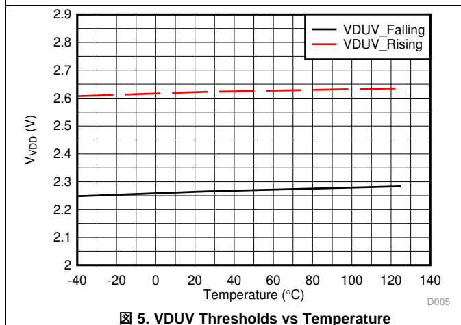
Figure 5. VDUV Thresholds vs Temperature
