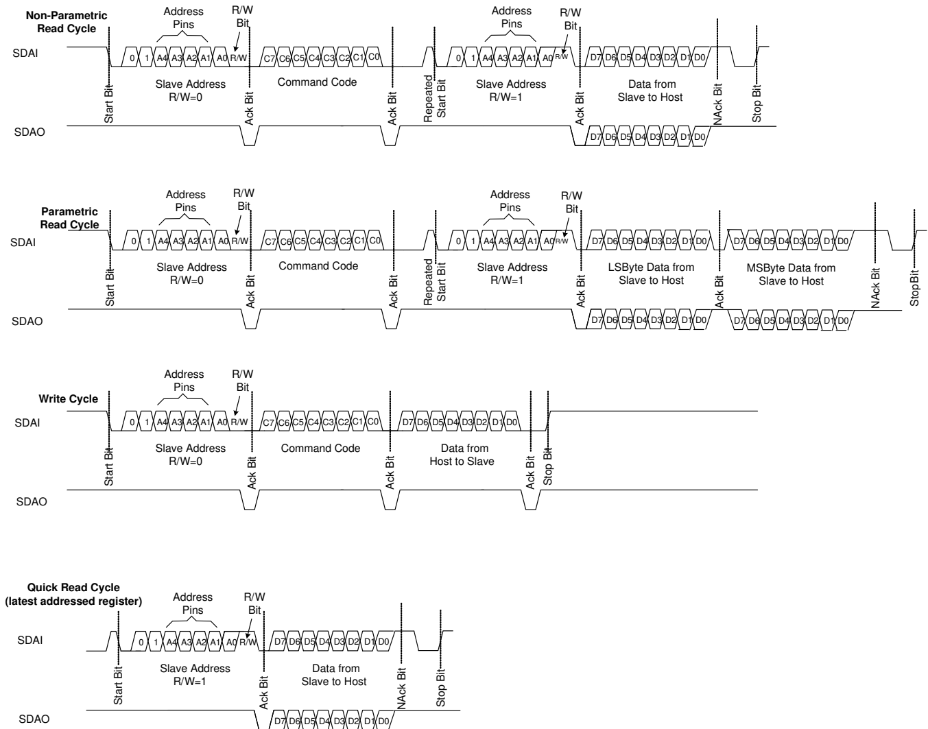
⊠ 43. I 2 C interface Read and Write Protocol – Configuration A
