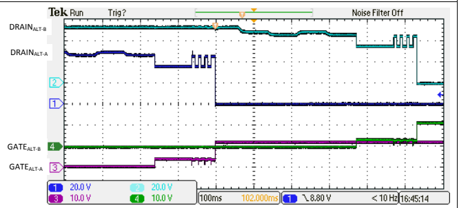
148. 4-Pair Dual Signature 4-Finger Classification and Turn On
