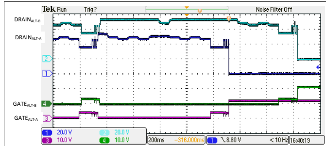
145. 4-Pair Dual Signature Discovery and Turn On from Semi-Auto Mode
