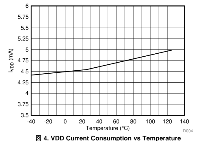
Figure 4. VDD Current Consumption vs Temperature
