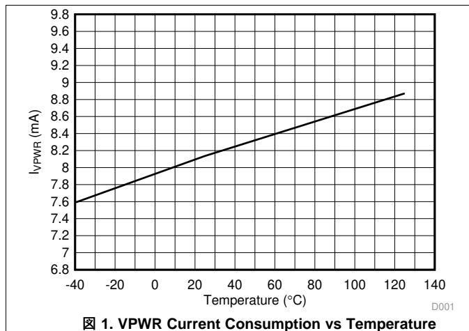
Figure 1. VPWR Current Consumption vs Temperature
