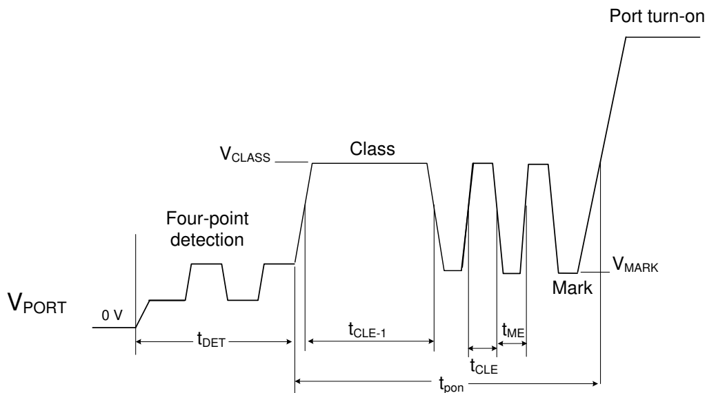
☒ 34. 2-Pair Detection, 3-Event Classification and Turn On
