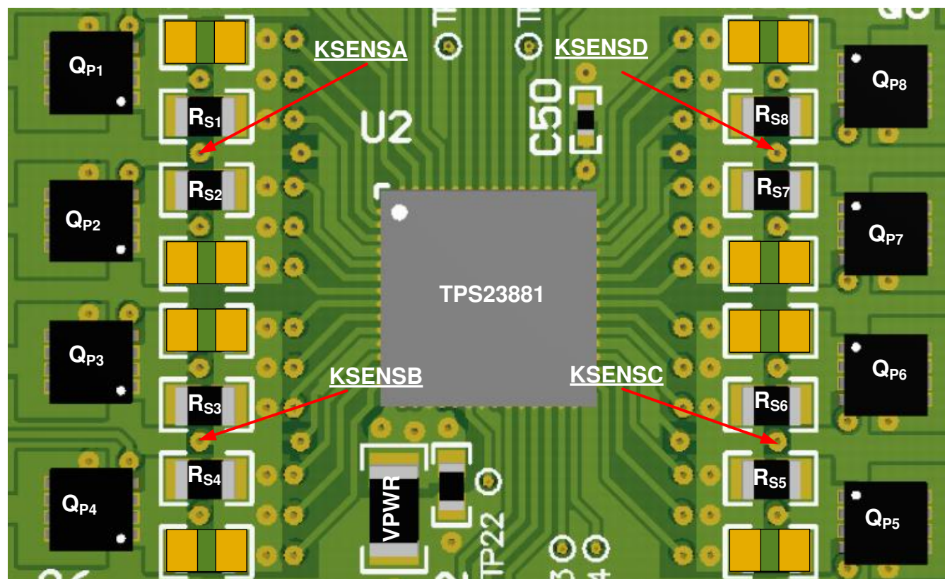
✎ 151. Eight Port Layout Example (Top Side)
