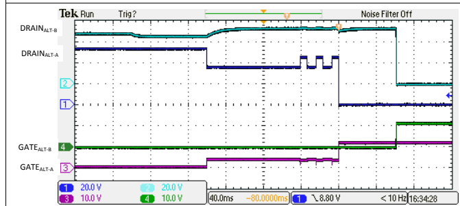
Figure 141. 4-Pair Single Signature 3-Finger Classification and Turn On
