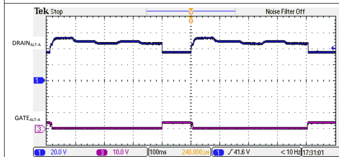
135. 2-Pair Semi-Auto Mode Discovery with a Valid Class 0-3 Load
