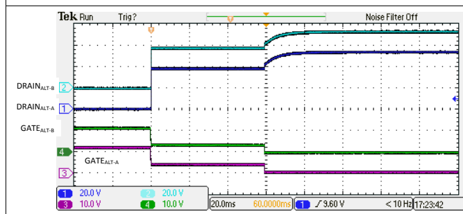
图 127. 4-Pair I_{LIM} Foldback and Turn Off
