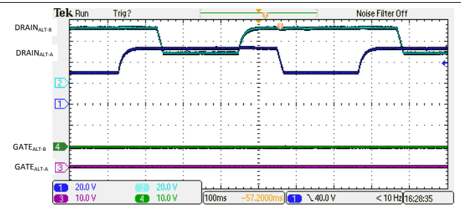
132. 4-Pair Open Circuit Detection Signature
