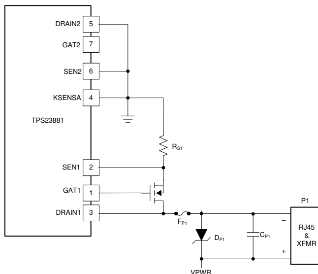
☒ 124. Unused PORT2 Connections
