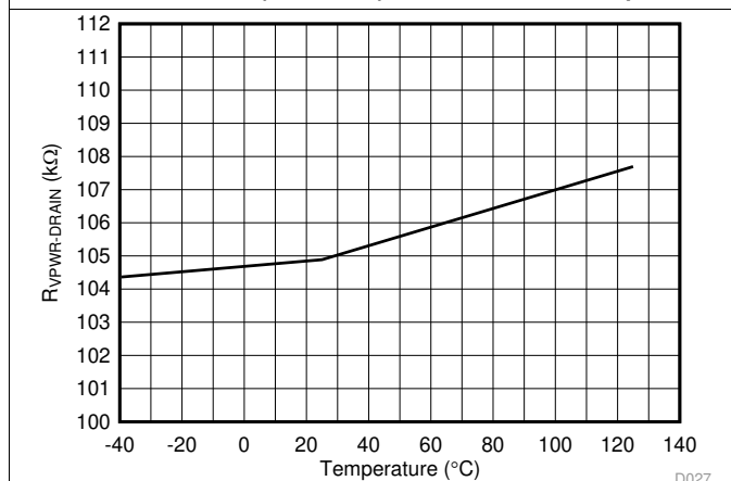
图 27. R_OFF (VPWR to DRAIN) vs Temperature
