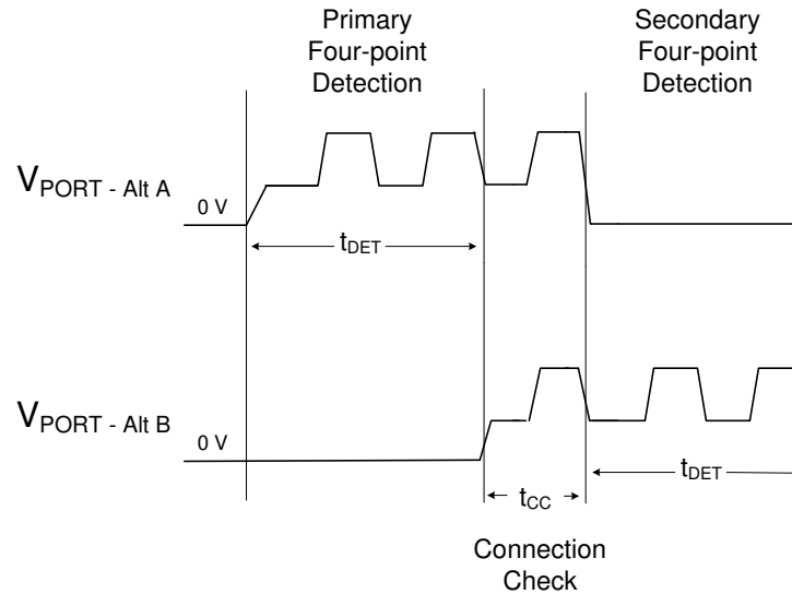
⊠ 41. 4-Pair Port, Detection and Connection Check Waveforms with a Single Signature Load
