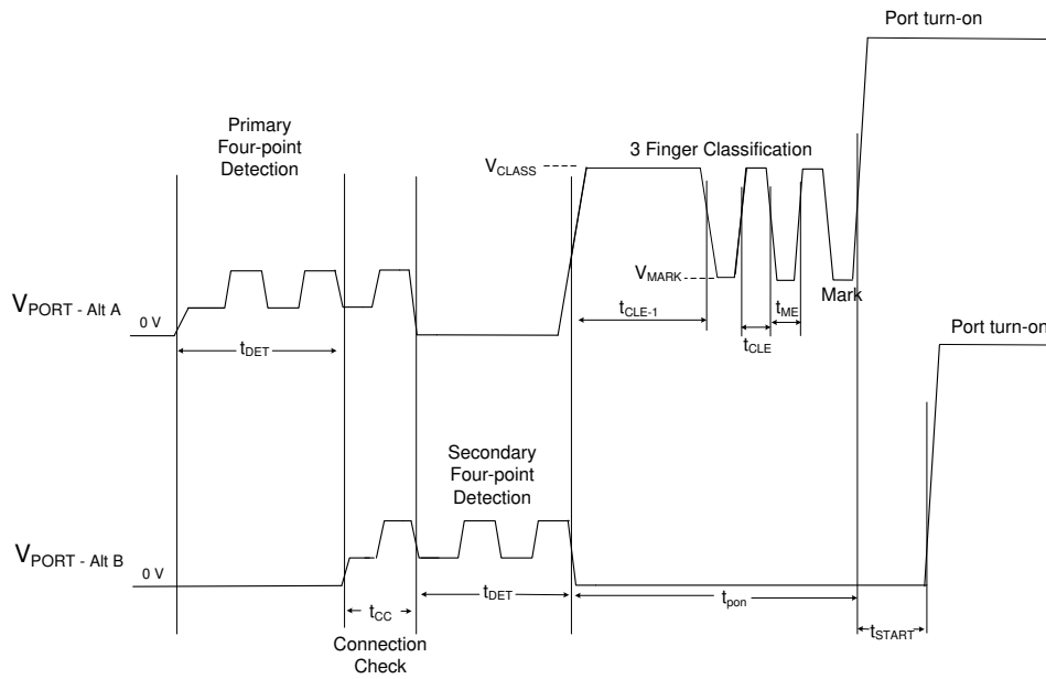
⊠ 35. 4-Pair Single Signature Detection, 3-Event Classification and Turn On
