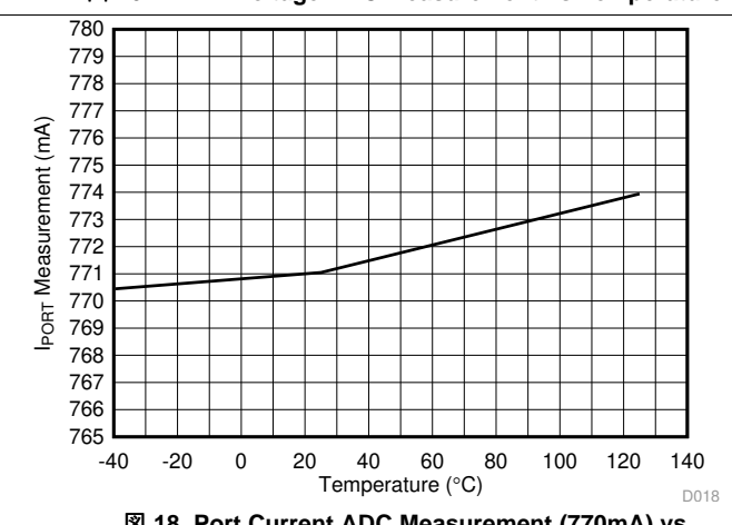
Figure 18. Port Current ADC Measurement (770mA) vs Temperature
