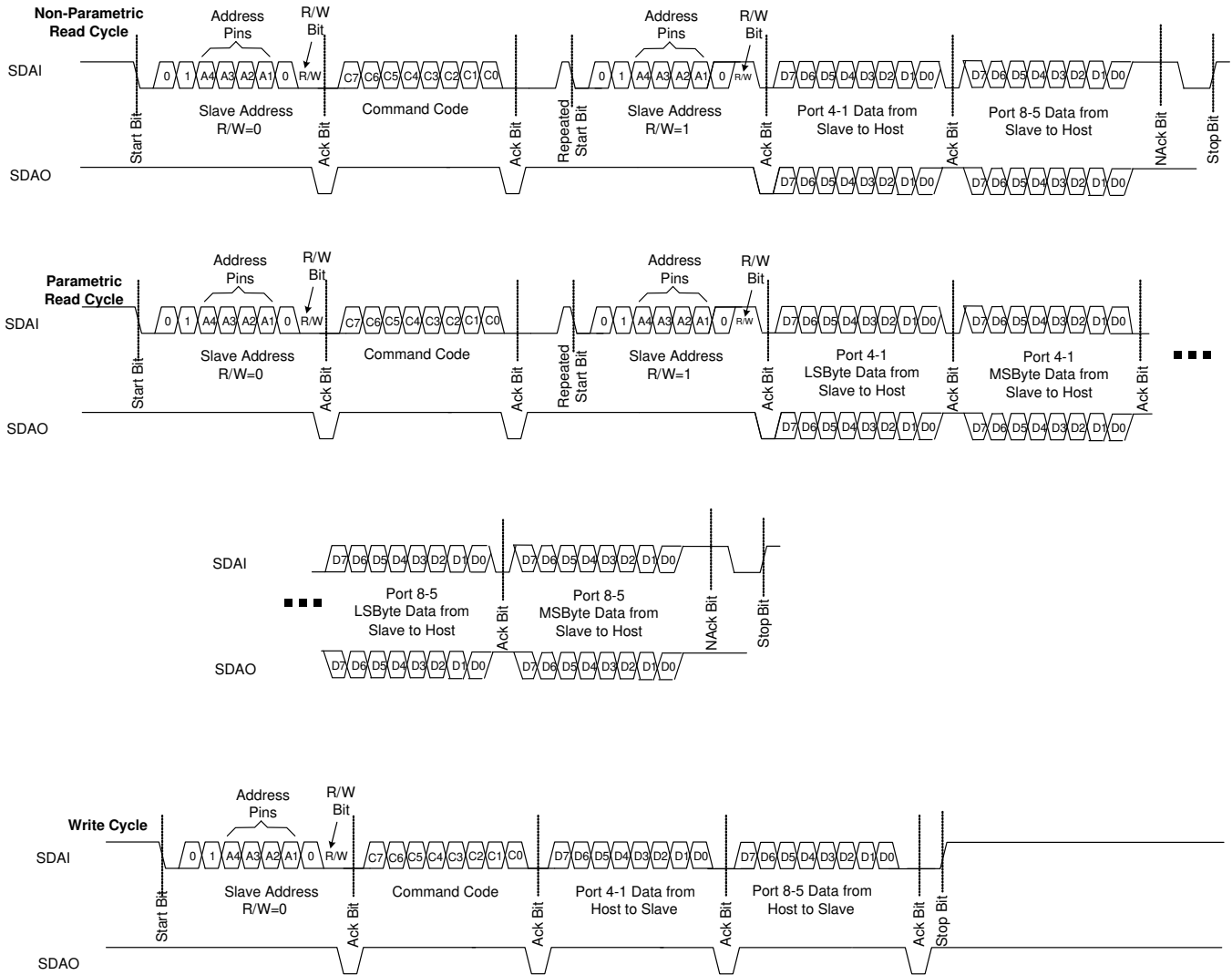
FIG 44. I 2 C interface Read and Write Protocol – Configuration B
