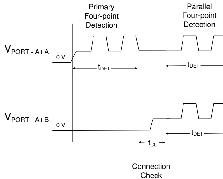
⊠ 42. 4-Pair Port, Detection and Connection Check Waveforms with a Dual Signature Load
