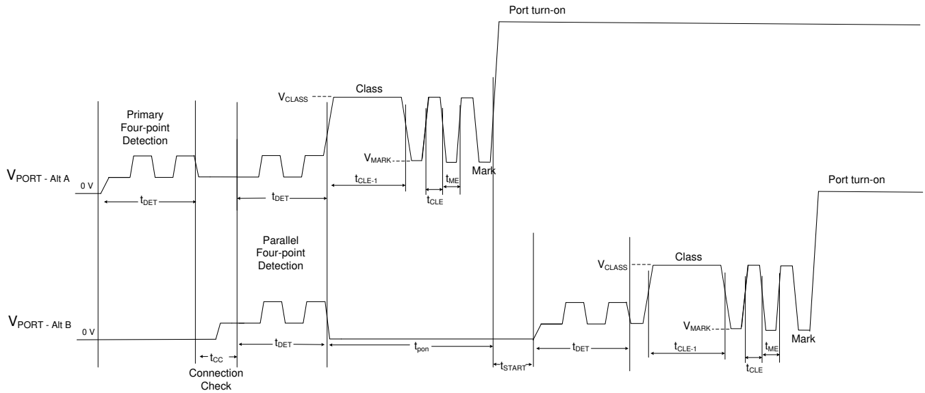
37. 4-Pair Dual Signature Detection, 3-Event Classification and Turn On
