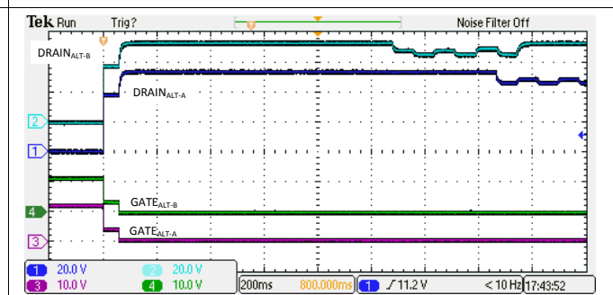
图 128. 4-Pair Backoff Due to I_{LIM} Fault
