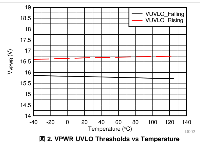
Figure 2. VPWR UVLO Thresholds vs Temperature
