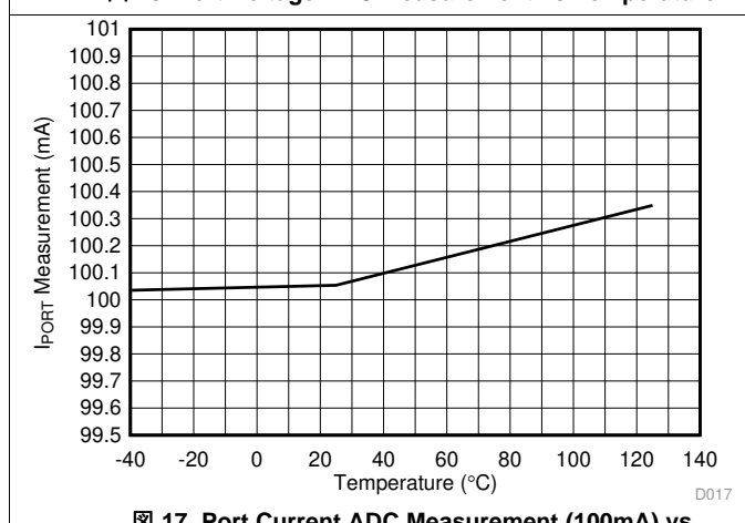
Figure 17. Port Current ADC Measurement (100mA) vs Temperature
