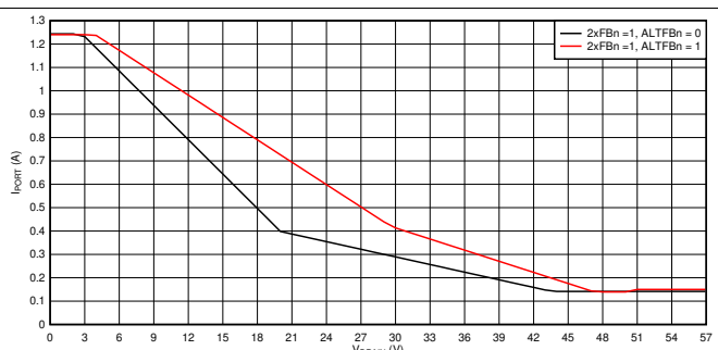
117. 2x Mode (2xFBn = 1) Foldback Curves, I PORT vs V DRAIN
