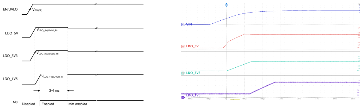
図 8-1. EN/UVLO and LDO Sequencing
