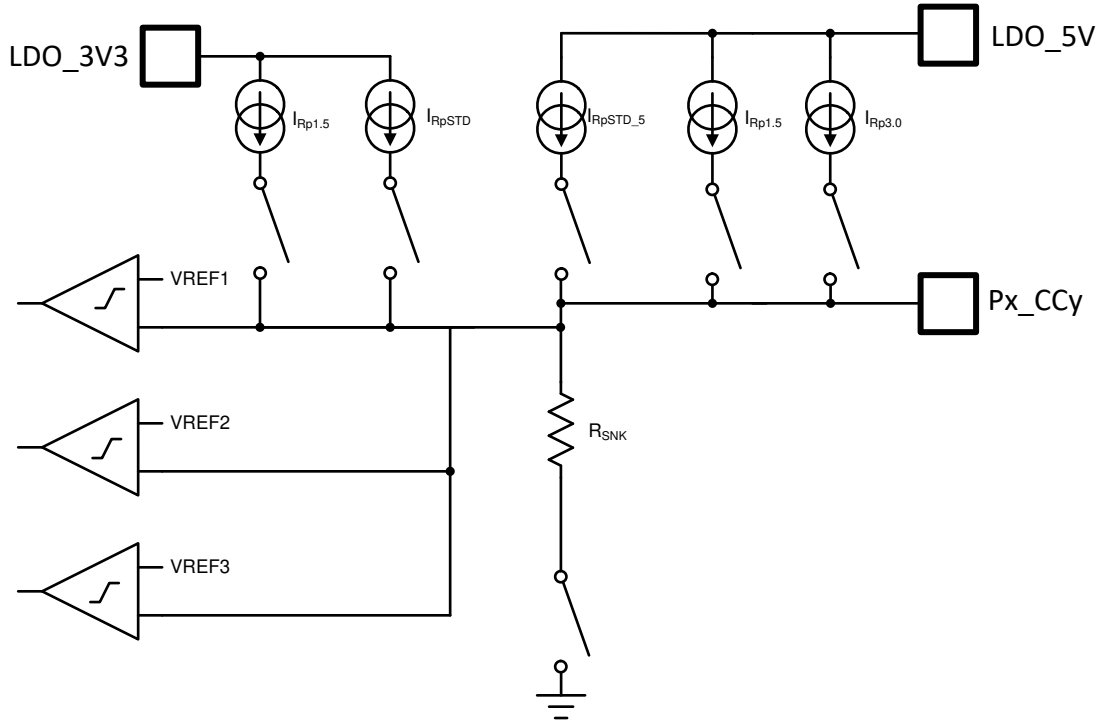
図 8-28. Plug and Orientation Detection Block
