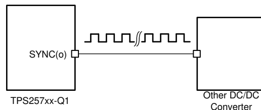
图 8-16. Using SYNC(o) to drive external DC/DC Converter
