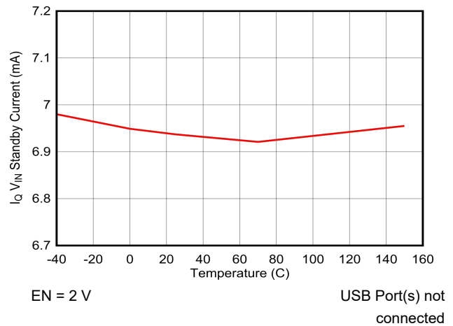
Figure 6-2. I_{Q\text{ VIN}} Standby Current vs Temperature
