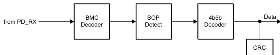
図 8-21. USB-PD Baseband Receiver Block Diagram
