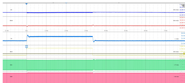
図 9-32. Load Transient (Buck-Boost): V_{BUS} = 15V
