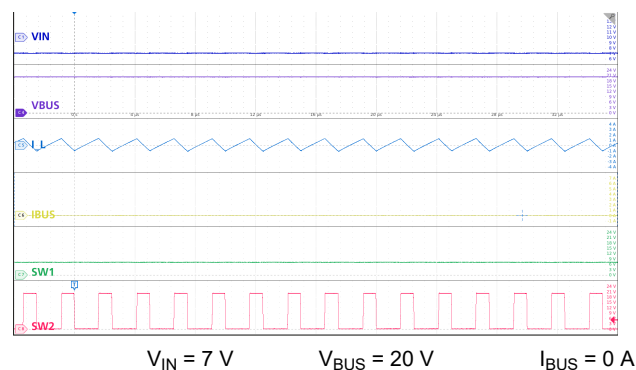
図 9-14. Boost Mode: Low V_{IN} , No Load
