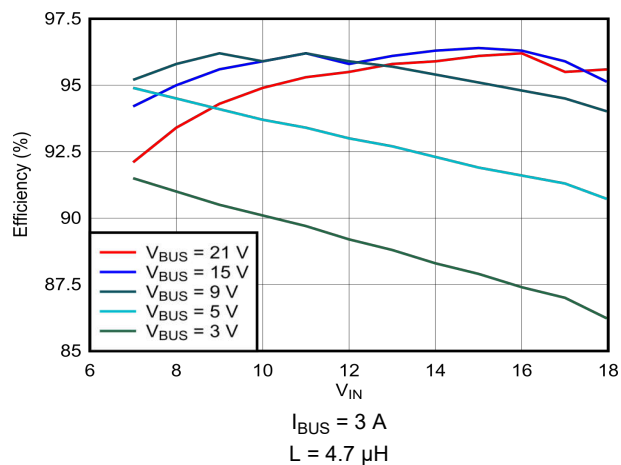
図 9-11. Efficiency vs Input Voltage
