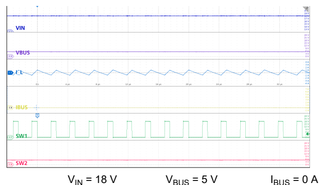
図 9-15. Buck Mode: High V_{IN} , No Load
