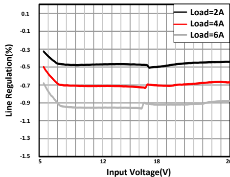
11-6. Line Regulation
