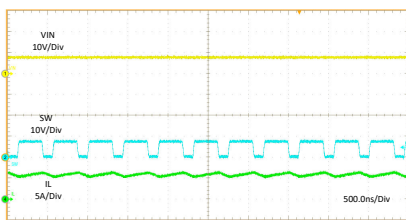
10-5. Switching Frequency When R_{FREQ} = 8.45 \text{ k}\Omega
