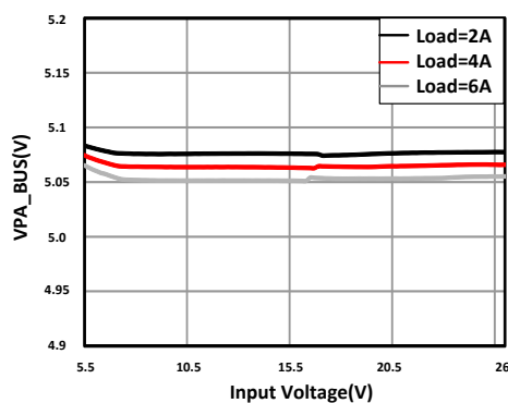
11-12. Dropout Characteristic
