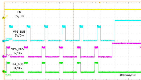
11-25. 1- \Omega Load Recovery
