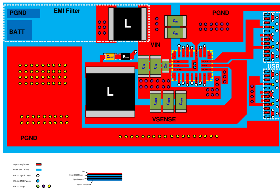
13-1. Layout Example
