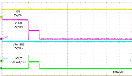
11-28. OUT short to 5.1-Ω Load
