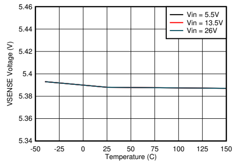
8-6. V_{SENSE} Voltage vs Junction Temperature
