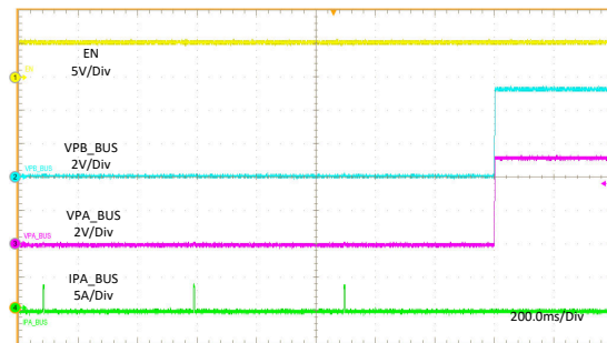
11-23. Short Circuit Recovery
