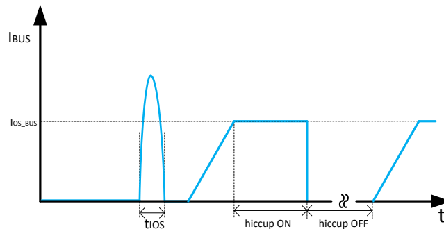
10-11. Response Time to BUS Short-Circuit
