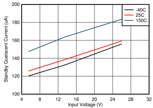
8-2. Standby Quiescent Current
