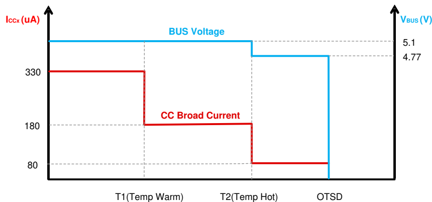
10-17. TPS25850-Q1 Behavior When Trigger Temp Warm/Hot Threshold
