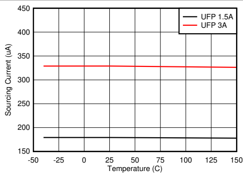
8-23. CC Sourcing Current vs Junction Temperature
