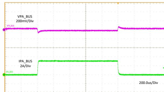
11-5. Load Regulation
