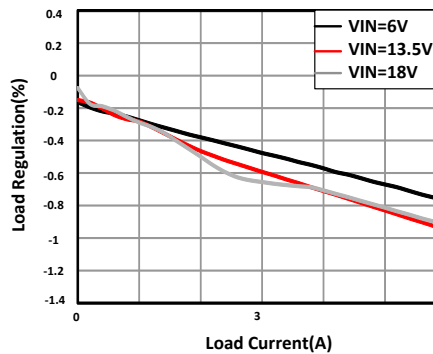
11-5. Load Regulation
