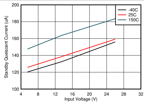
FIG 8-2. Standby Quiescent Current
