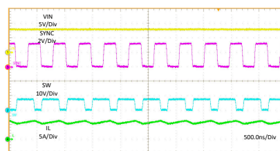
FIG 10-6. Switching Frequency When R_{FREQ} = 8.45 \text{ k}\Omega
